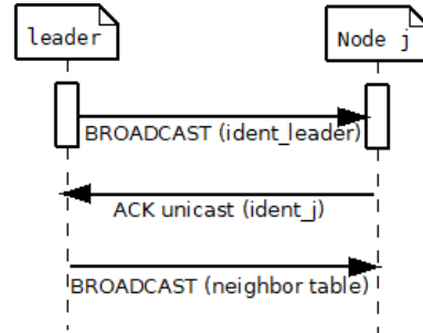
Fig. 1. Leader-based protocol
