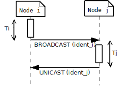
Fig. 2. TDMA-based proposal.
