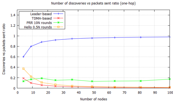
Fig. 10. Discoveries vs total packets sent ratio (collisionModel 2).
