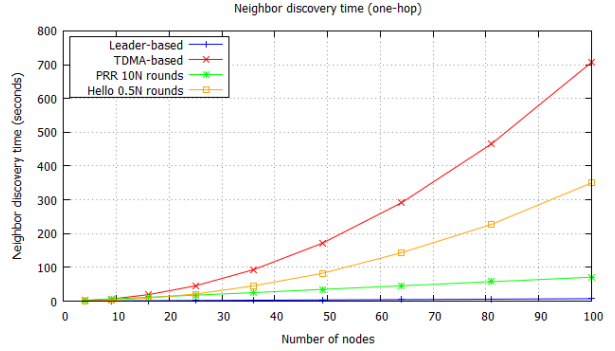
Fig. 4. Neighbor Discovery Time (collisionModel 2).
