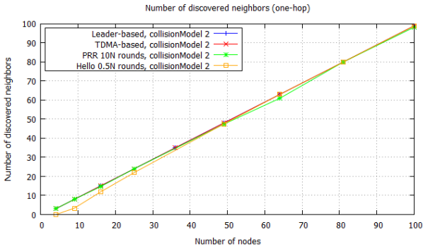
Fig. 7. Number of discovered neighbors (collisionModel 2).
