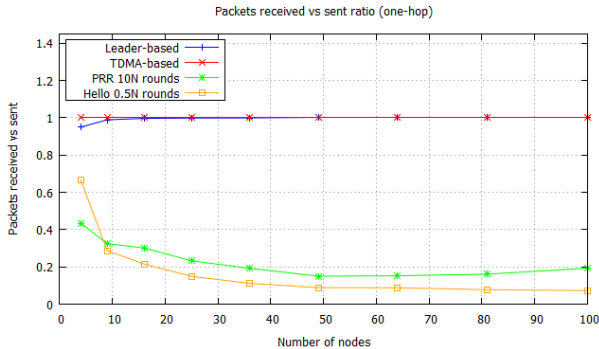
Fig. 11. Packets received vs packets sent ratio (collisionModel 2).
