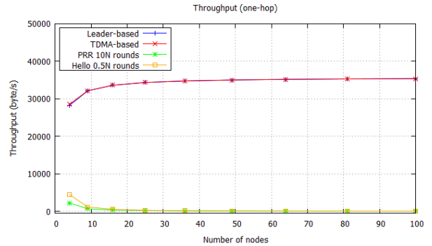
Fig. 9. Average Throughput per node (collisionModel 2).
