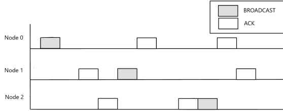
Fig. 3. TDMA-based protocol (timeline).
