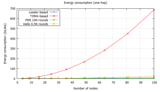
Fig. 8. Average Energy consumption per node (collisionModel 2).
