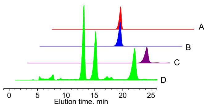
Figure 3. HPLC chromatograms obtained for A) DMDP, B) photoproduct 2 , C) photoproduct 1 , D) UVC irradiated sample (6 minutes at 254 nm, PBS/ \text{N}_2 , 5 mg/mL). The obtained samples were esterified before analysis (see Section 2.4).
