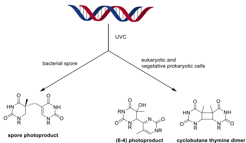
Chart 1. Structures of spore photoproduct (SP) and cyclobutane thymine dimers (CPD) and (6-4) photoproduct (6-4PP).
