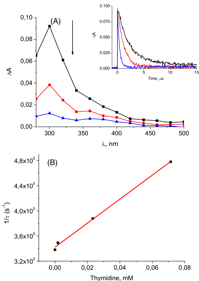
Figure 4. (A) Transient absorption spectrum of DMDP in deaerated MeCN:H 2 O (1:9, v:v) from 0.4 to 9 \mu s after the 266 laser pulse. Inset: decay monitored at 300 nm under N 2 (black), air (red) or O 2 (blue) atmosphere. (B) Stern-Volmer representation for the quenching of 3 DMDP* by Thd.
