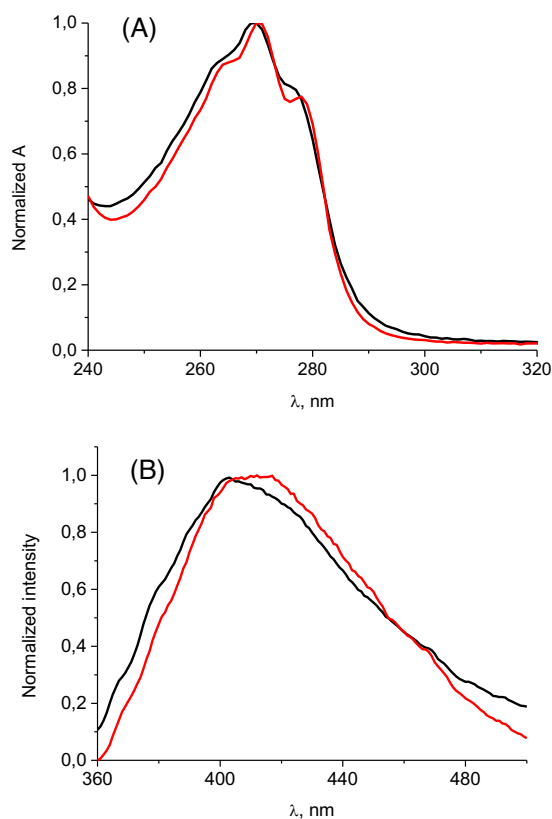
Figure 1. (A) Normalized UV absorption spectra of DPA (black line) in PBS and DMDP (red line) in H 2 O:MeCN (9:1), (B) Phosphorescence spectrum ( \lambda_{exc}=266 nm) of DPA (black line) and DMDP (red line) in EtOH at 77K.
