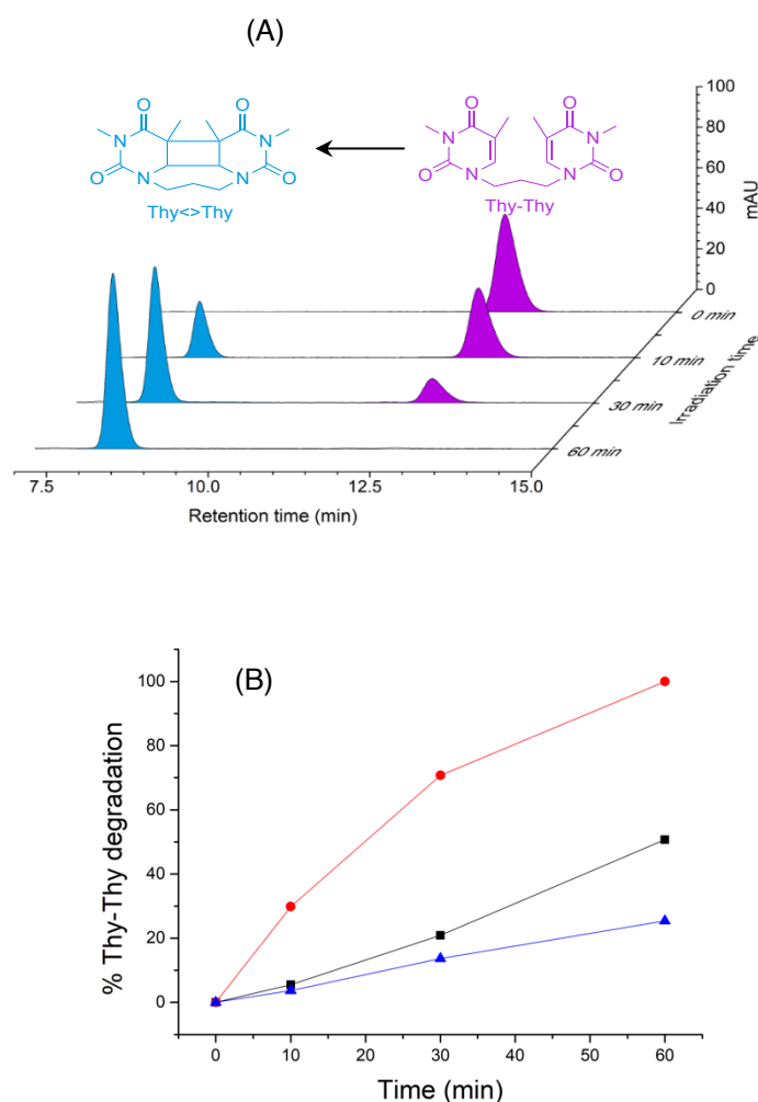
Figure 8. A) HPLC chromatograms recorded at 240 nm for a solution of Thy-Thy: 1 (0.5 mM:1.5 mM) in H 2 O:MeCN (1:1, v:v) irradiated at 300 nm. B) Time-dependent photodegradation of Thy-Thy UVB-irradiated in the presence of DMDP (black), 1 (red) and alone (blue).
