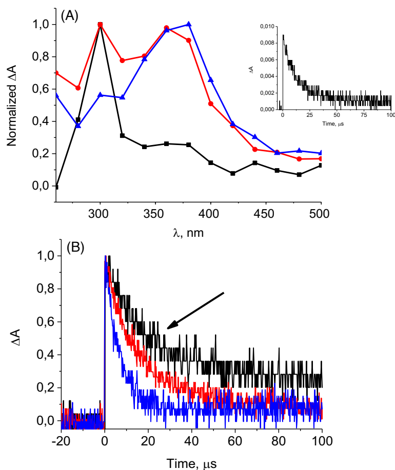
Figure 2. (A) Transient absorption spectra of \text{N}_2 degassed PBS solution of DPA obtained changing the sample after each pulse/wavelength record, using fresh ( \blacksquare ), one pulse ( \bullet ) or two pulses ( \blacktriangle ) pre-irradiated solution. Inset: corresponding decay of DPA monitored at 300 nm. (B) Decays monitored at 300 nm for deaerated PBS solution of DPA in the presence of increasing amounts of Thd (0, 6.2 and 20 \mu\text{M} ).
