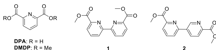
Chart 2. Chemical structures of dipicolinic acid ( DPA ), its methyl ester derivative ( DMDP ), photoproducts 1 and 2 .
