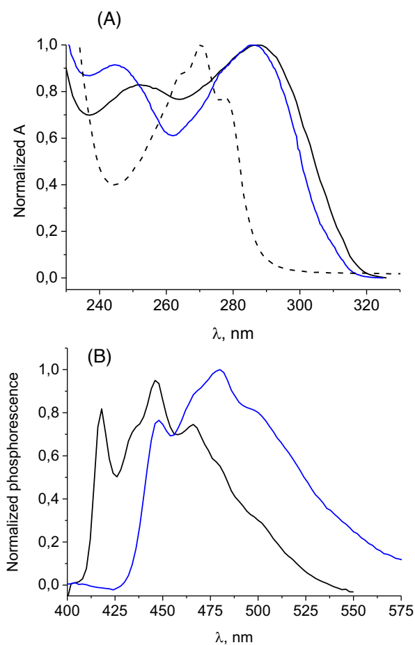
Figure 5. A) Normalized absorption spectra of photoproducts 1 (black line) and 2 (blue line) in PBS, DMDP spectrum (dash line) is given for comparison B) Normalized phosphorescence emission spectra ( \lambda_{exc}=300 nm) of photoproducts 1 (black line) and 2 (blue line) in EtOH.
