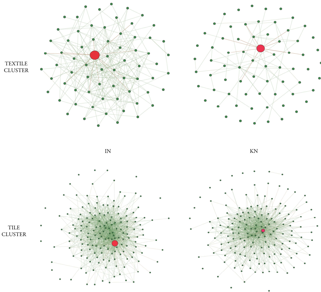
FIG. 2. Network Graphs
