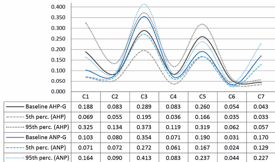
Figure 3. Dispersion in the weightings of the criteria with AHP and ANP.
