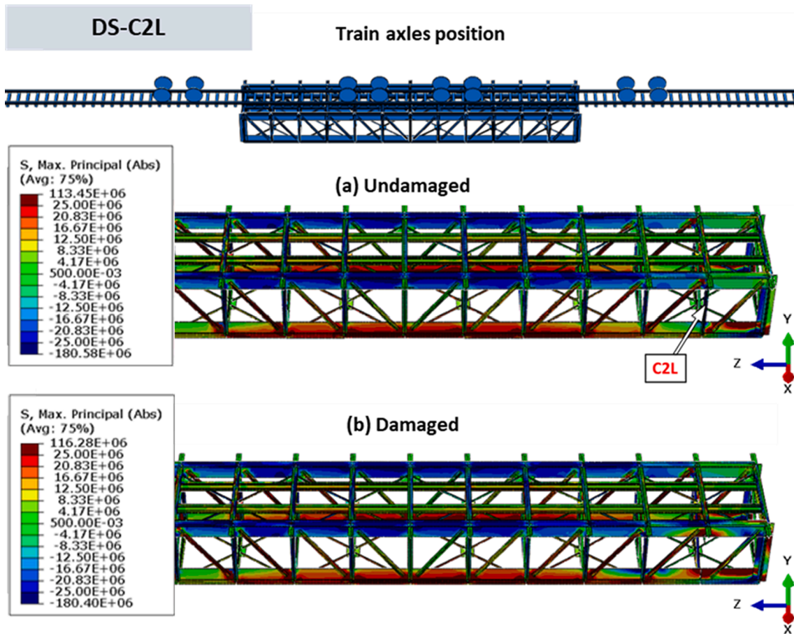
Fig. 22. DS-C2L: Principal stress contour maps obtained considering undamaged (a) and damaged (b) states. Units in Pa.
