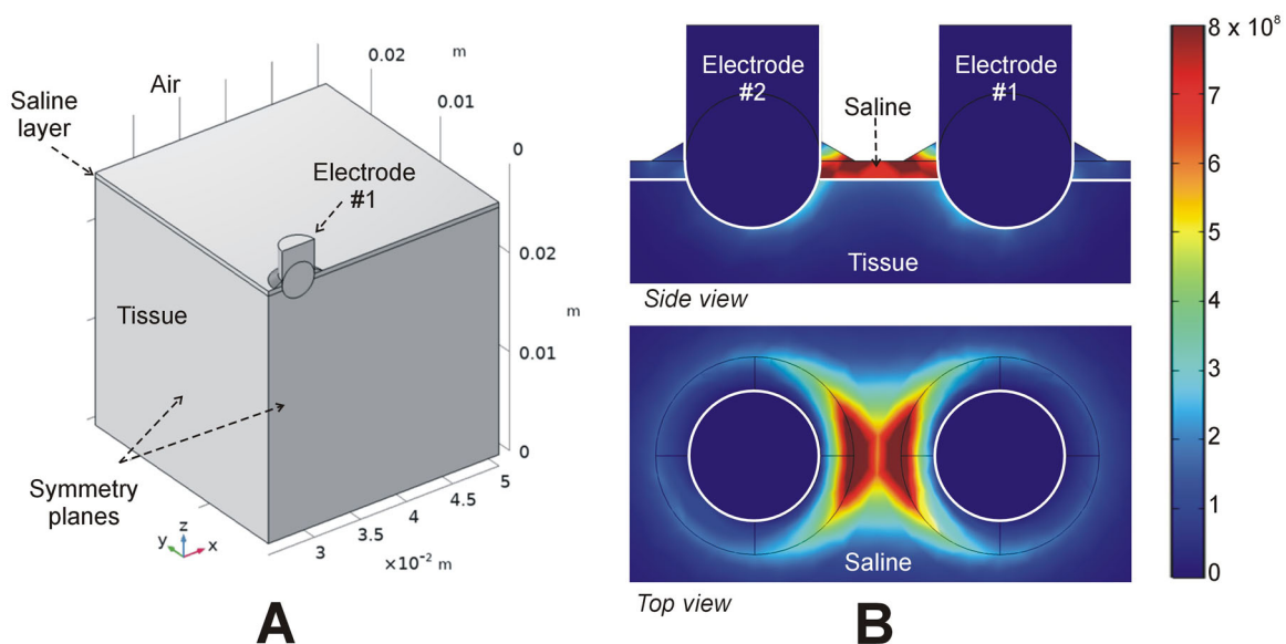
Figure 4. In-silico modeling of the Aquamantys device. (A) Geometry of the 1/4 scale 3D model using two symmetry planes. (B) Electrical power density (in \text{W/m}^3 ) deposited in saline and tissue at 20 W power.
