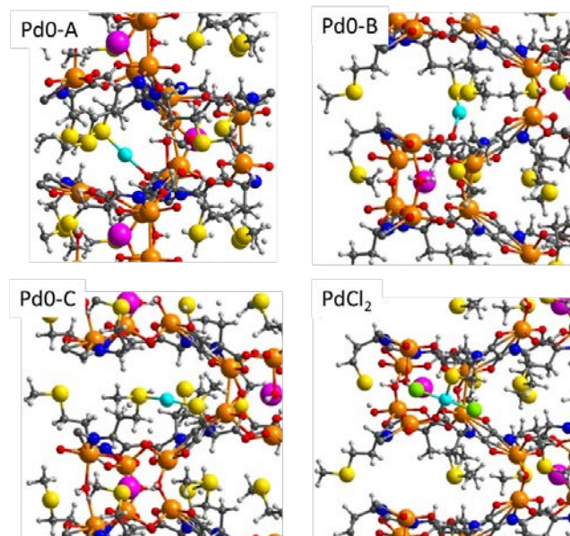
Figure 7. DFT optimized structures of Pd(o) and PdCl 2 within the MOF, for three different coordination environments (PdO-A-C, see also Figure S20 and Table S5). Pd, Cu, Sr, S, N, O, Cl, C and H atoms are depicted as cyan, orange, pink, yellow, blue, red, green, grey and white balls, respectively.
