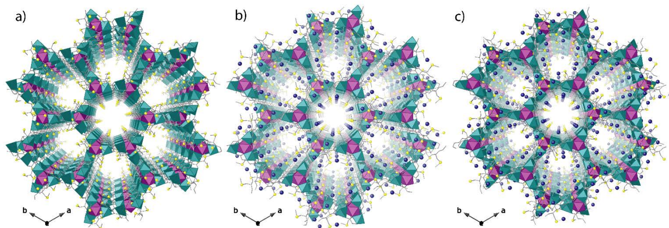
Figure 3. PS approach showing the structures of 3–5 determined by single-crystal X-ray diffraction which consists of two consecutive processes. First, the insertion of [\text{Pd}(\text{NH}_3)_4]^{2+} cations within the channels of 3 (a) to give 4 (b) and second the reduction of \text{Pd}^{2+} cations to form the \text{Pd}^0 , single atoms in 5 (c). Copper and strontium atoms from the network are represented by cyan and purple polyhedra, respectively, whereas organic ligands are depicted as gray sticks. Yellow and blue spheres represent S and Pd atoms. Dotted lines represent the \text{Pd}\cdots\text{S} interactions
