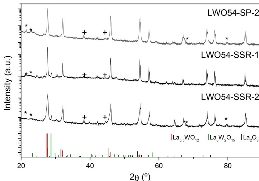
Fig. 8. Room temperature XRD patterns of LWO54-SSR-1, LWO54-SSR-2 and LWO54-SP-2 as bars after the conductivity measurements (peaks corresponding to sample holder and silver used for the contacts are indicated as * and +, respectively). \text{La}_{5.5}\text{WO}_{12} , \text{La}_6\text{W}_2\text{O}_{15} and \text{La}_2\text{O}_3 patterns were included for comparison.
