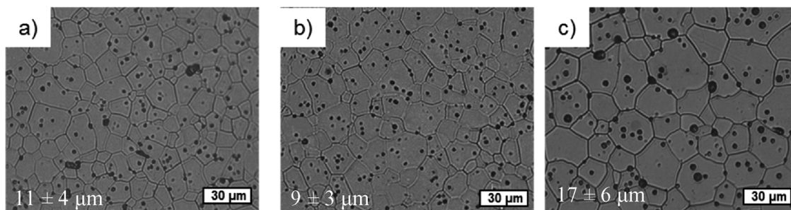
Fig. 12. Microstructures of dense LWO54 specimens: (a) LWO-SSR-1, (b) LWO-SP-1 (c) LWO-SP-2.
