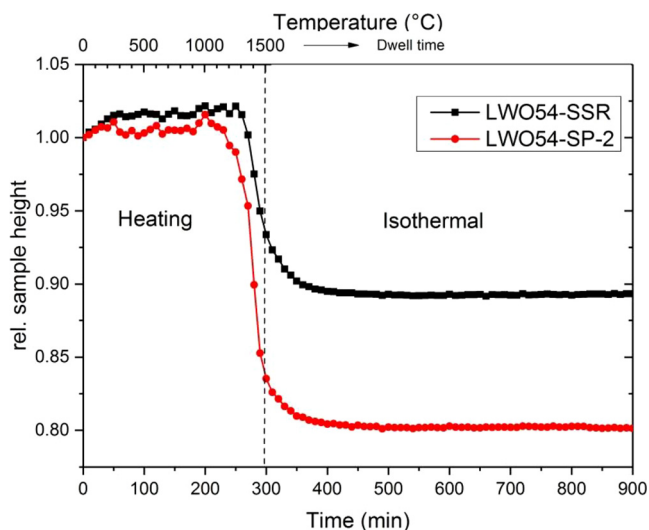
Fig. 2. Shrinkage of pressed LWO54-SSR and LWO54-SP-2 powders sintered at 1500 °C for 10 h.
