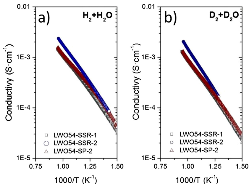
Fig. 7. Total conductivity comparison of the three LWO54 samples with different grain size as a function of reciprocal temperature in (a) H 2 +H 2 O and (b) D 2 +D 2 O atmospheres (H 2 and D 2 diluted in 95% He).
