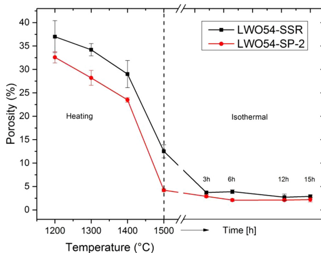
Fig. 3. Porosity of LWO54-SSR and LWO54-SP-2 pellets during sintering at 1500 °C for 15 h obtained by SEM image analysis.
