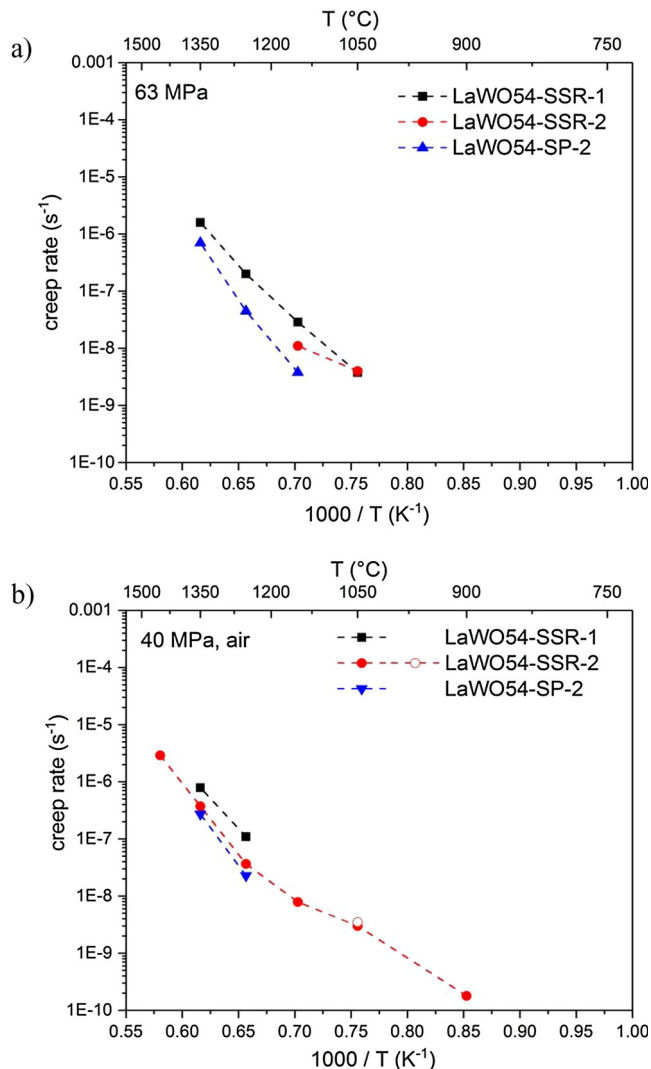
Fig. 14. Arrhenius plots for LWO54 materials with applied stresses of 63 MPa (a) and 40 MPa (b) in air. (For interpretation of the references to colour in the text, the reader is referred to the web version of this article.)
