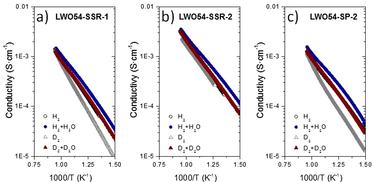
Fig. 6. Total conductivity for LWO54-SSR-1, LWO54-SSR-2 and LWO54-SP-2 samples as a function of reciprocal temperature in H 2 , D 2 , H 2 +H 2 O and D 2 +D 2 O atmospheres (H 2 and D 2 diluted in 95% He).
