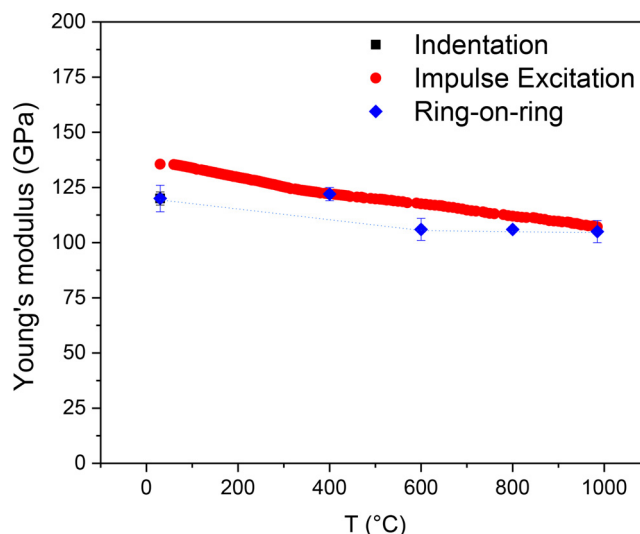
Fig. 10. Evolution of Young's modulus with temperature for LWO54-SP-1 tested with impulse excitation and Ring-on-Ring method.
