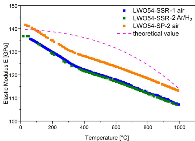
Fig. 9. Elastic modulus of LWO54 in air (LWO54-SSR-1 and LWO-SP-2) and in Ar/4% \text{H}_2 (LWO54-SSR-2) as a function of temperature measured by the impulse excitation technique. The dashed lines represent the model from Hillig.
