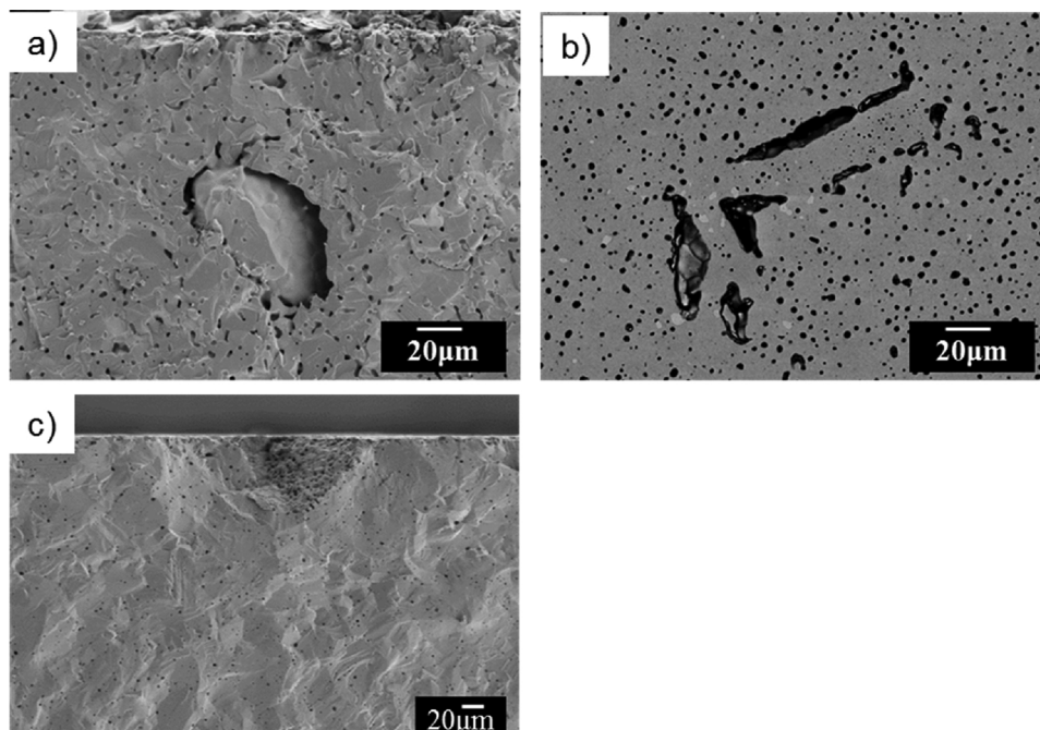
Fig. 11. Microstructure of LWO54-SP1 showing agglomerates as failure origin in a fracture surface \sigma_B = 44 MPa (a) and irregular pores and agglomerate in the polished cross section (b). LaWO54-SP-2 failure origin is a pore zone (c).
