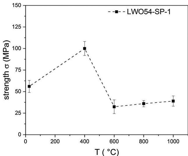
Fig. 13. Dependence of strength on temperature (LWO54-SP-1 batch) at temperatures up to 1000 °C.
