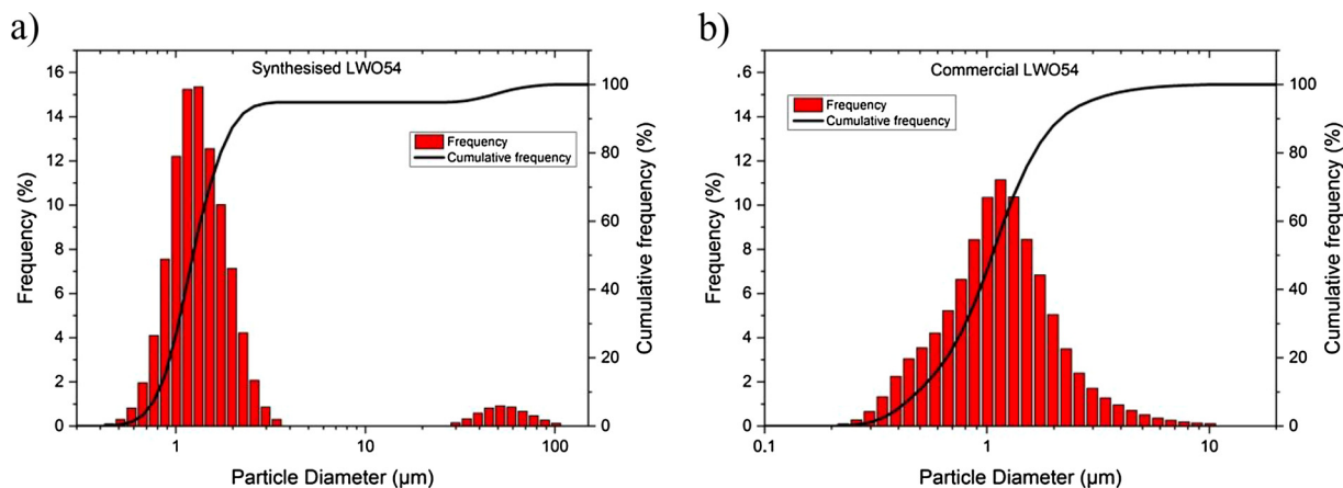
Fig. 1. Particle size distribution of (a) the in-house synthesized LWO54-SSR-1 powder and (b) the commercial LWO54-SP-2 powder calcined at 1100 °C.
