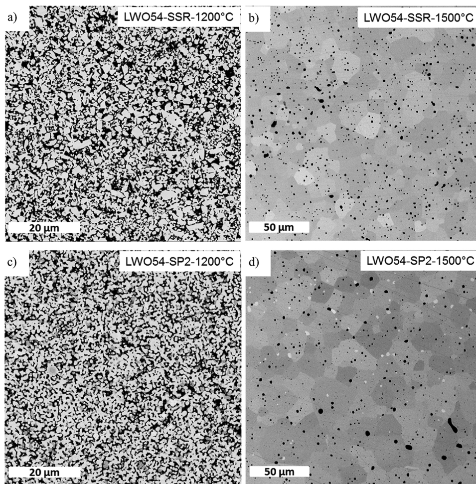
Fig. 4. Microstructure of pressed specimens after sintering at 1200 °C and 1500 °C and 15 h holding time. (a) LWO54-SSR 1200 °C; (b) LWO54-SSR 1500 °C, 15 h; (c) LWO54-SP-2 1200 °C; (d) LWO-SP-2 1500 °C, 15 h.
