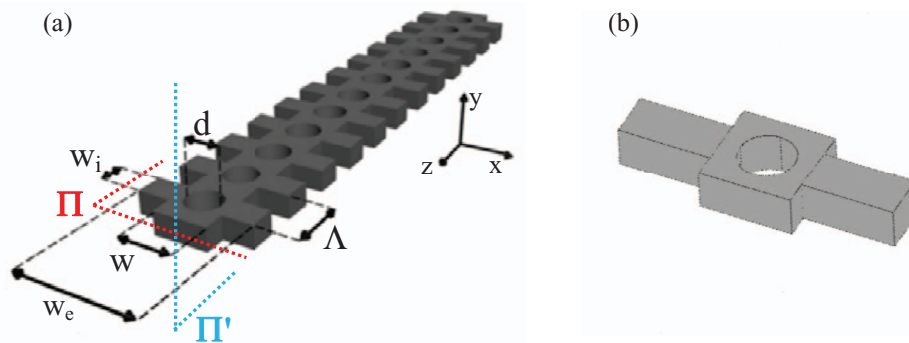
FIG. 1. (a) Schematic view of the periodic silicon strip waveguide. (b) Representation of the unit cell which contains one hole in the middle of the waveguide and two symmetric stubs on each side.
