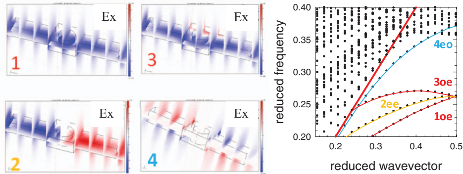
FIG. 4. Map of the x component of the electric field for the lowest four modes in Fig. 3(b) at the reduced wavenumber k\Lambda/2\pi=0.414 .
