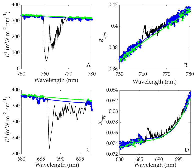
Figure 4. Example of correct (green) and incorrect (blue) implementation of polynomial second-order interpolation for the down-welling irradiance ( E^{\downarrow} , A,C) and cubic spline interpolation for the apparent reflectance ( R_{app} , B,D) at O 2 B (F 687 , C,D) and O 2 A (F 760 , A,B) bands.
