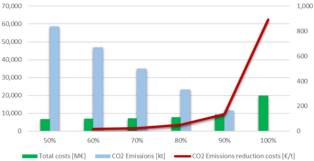
Figure 10 Economic and environmental metrics under different decarbonisation objectives
