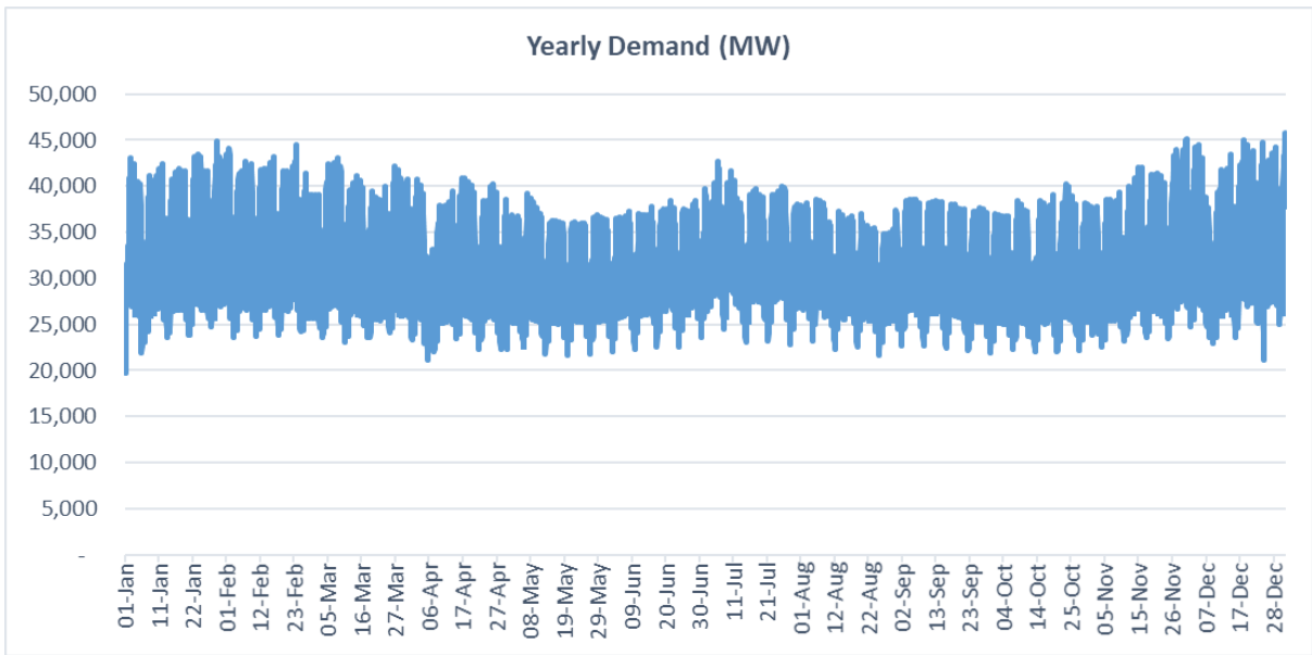
Figure 13 Demand profile of one of the weather years simulated
