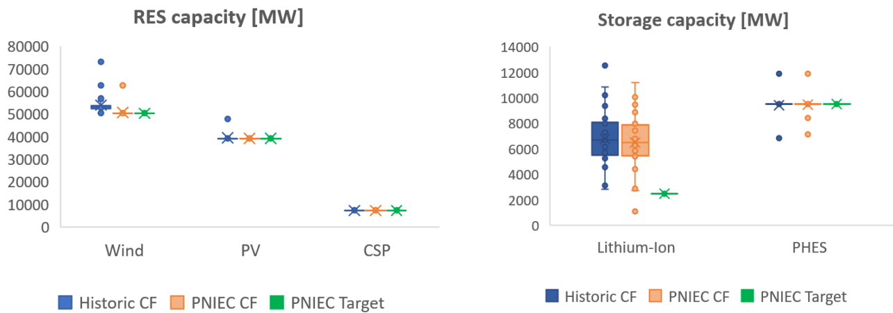
Figure 6 Sensitivity analysis of the installed RES and energy storage capacity considering the PNIEC’s RES installed capacity as a minimum
