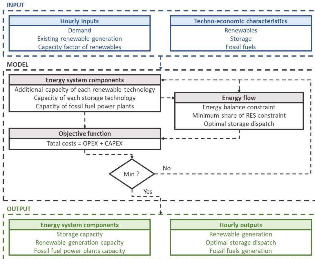
Figure 1 Simplified model flow chart.
