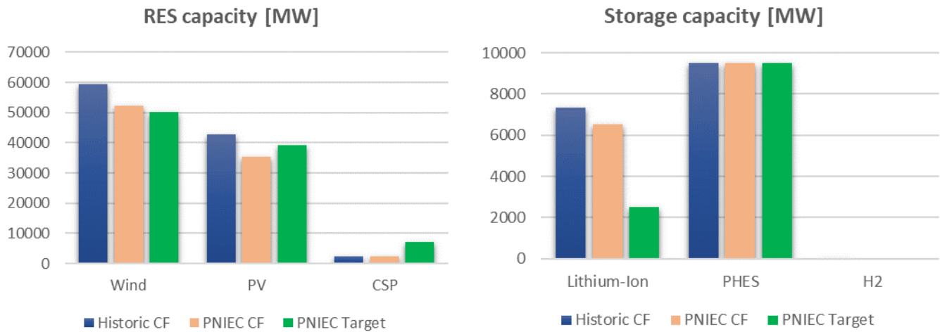
Figure 5 Results of the installed capacity under the base scenarios with different capacity factors
