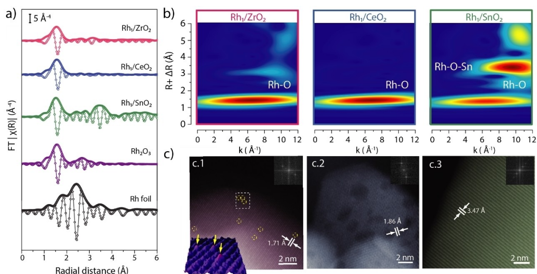
Figure 2. Structural analysis of Rh single-atom catalysts on different oxide support materials. a) Fourier Transform of the k^3 -weighted EXAFS function (no phase correction) and b) Continuous Cauchy Wavelet Transforms of the EXAFS function for the series of as-synthesized \text{Rh}_1/\text{MO}_2 catalysts ( M = \text{Zr}, \text{Ce}, \text{Sn} ). For reference purposes, data for \text{Rh}_2\text{O}_3 (dispersed on carbon) and a metallic Rh foil are also included on panel (a). The spectra were collected at room temperature under He for the as-synthesized catalysts, i.e. following Rh incorporation on the oxide supports and oxidative metal dispersion in air at 1073 K. c) Representative AC-HAADF-STEM images. Insets (top-right) show the Fast Fourier-Transform function applied to determine the crystal d -spacings indicated on the micrographs, which correspond to the (2 0 2) plane in m - \text{ZrO}_2 (c.1), (2 2 0) in \text{CeO}_2 (c.2) and (1 1 0) in \text{SnO}_2 (c.3), respectively. On panel (c.1) isolated Rh atoms have been marked by the dashed yellow circles included as a guide to the eye. The corresponding 3D map of Z-contrast for the region marked on the micrograph is also given, wherein the arrows point to the atomic-size high-Z-contrast objects ascribed to isolated Rh atoms.
