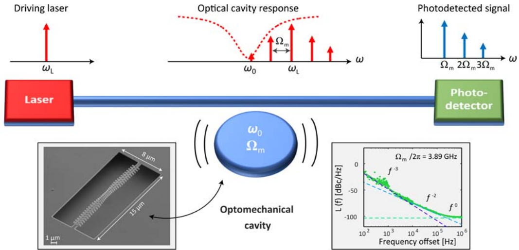
Figure 1: Conceptual scheme of an OMO. A laser, which generates coherent light at \omega_L , drives an OM cavity to the phonon lasing regime, which modulates the light exiting the cavity with tones at frequencies \omega_L \pm m \times \Omega_m . Upon photodetection, a low-noise signal at \Omega_m , as well as at integer multiples of it, is obtained. Left-side inset: scanning electron image of the silicon OM crystal cavity used in [13]. Right-side inset: phase noise of the cavity in [13] operating as an on-chip OMO. Green dots correspond to experimental data and dashed lines to fits to the different expected noise contributions: flicker white phase noise in light-green ( f^0 ), random walk of phase in light-blue ( f^{-2} ) and flicker frequency noise in dark-blue ( f^{-3} ).
