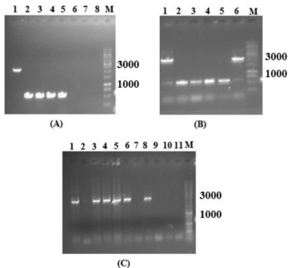
Figure 3 Agarose gels' electrophoresis of NzyTech PCR products from possible V5 HXT6/HXT7 transformants. (A) V5-HXT6-402 (1), not transformed V5 (2-5), not amplified colonies (6 and 7), MQ water negative control (8). (B) V5-HXT7-BC187 (1,6), not transformed V5 (2-5). (C) V5-HXT7-S288c (1,3,4,5,6,8), not transformed V5 (2,7,9) and V5 and mQ water negative controls (10,11). In all gels M: base pair marker (bp) of 1 kb.
