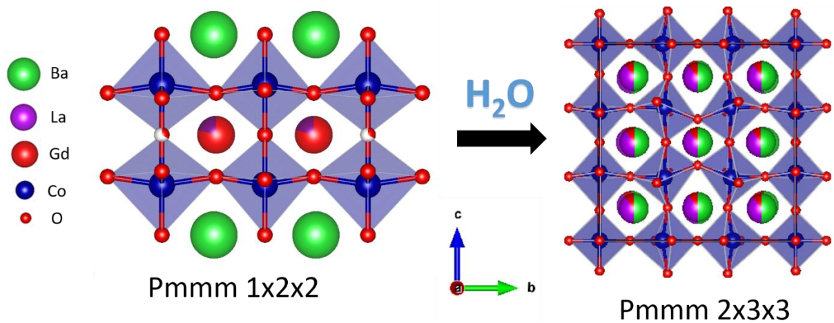
Figure 9: Proposed order-disorder transition of BGLC82 upon hydration.
