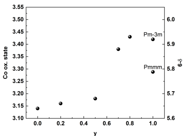
Figure 6: Cobalt oxidation state and oxygen non-stoichiometry versus y in BGLC ( x = 0, y = 0-1 ).
