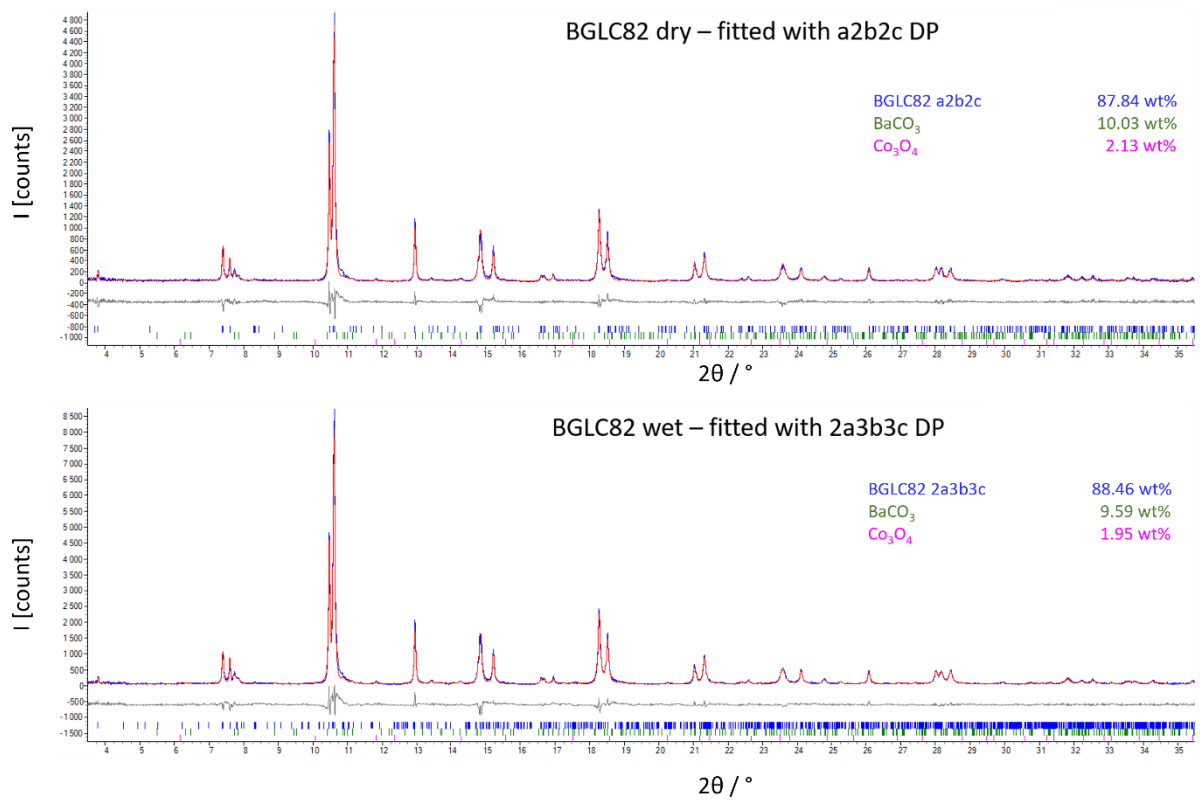
Figure 8: SR-PXD of BGLC82 treated in dry (upper) and wet (lower) atmosphere at 300°C. The spectra are fitted to a Pmmm a2b2c (dry), and a Pmmm 2a3b3c (wet) unit cell.
