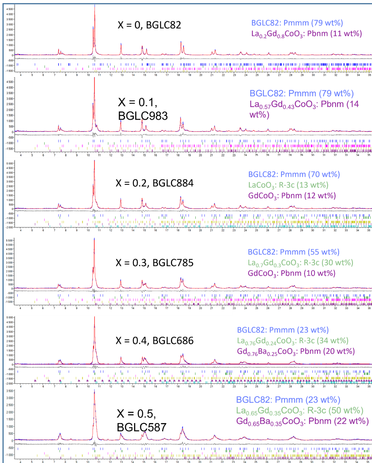
Figure 2: SR-PXD Rietveld refinements (red line) of BGLC ( x = 0-0.5 , y = 0.2 ). Minority phases \text{Co}_3\text{O}_4 , \text{Gd}_2\text{O}_3 and \text{BaCO}_3 are refined, but omitted in the figure legends.
