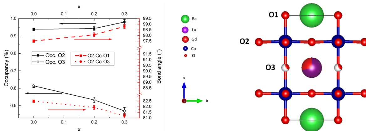
Figure 7: SR-PXD data at room temperature showing occupancies on O2 and O3 sites (left axis) and shift in O2-Co-O1 and O2-Co-O3 bond angles (right axis) with increasing La substitution x.
