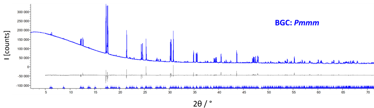
Figure 1: PND diffractogram of BGC with Rietveld refinement to orthorhombic Pmmm .
