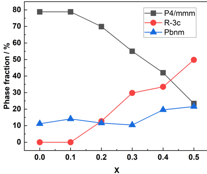
Figure 3: Phase fractions (wt%) vs x in BGLC ( y = 0.2 ).
