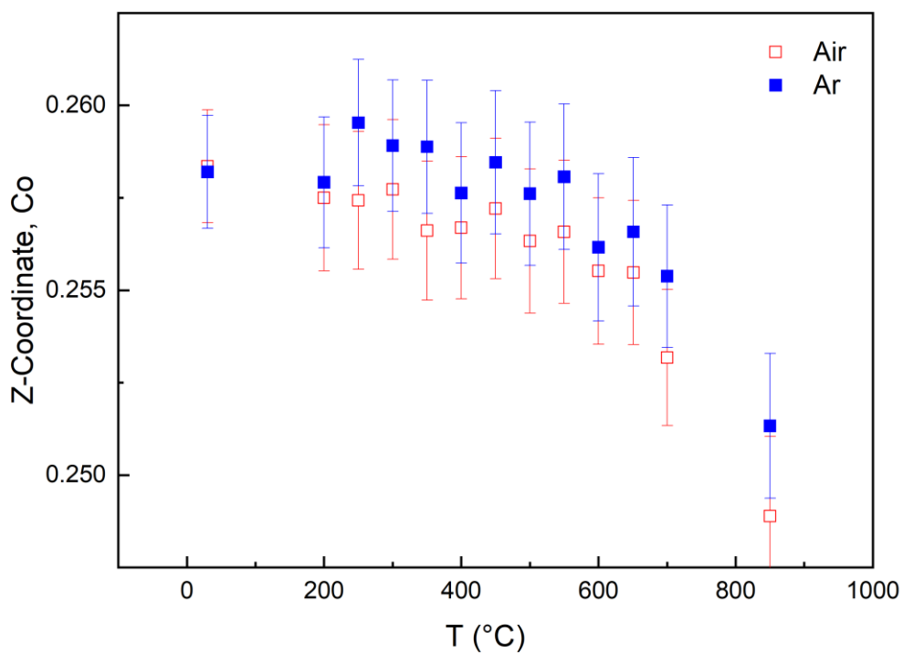
Figure 16: Z-coordinate of Co in BGLC ( x = 0, y = 0.2 ) upon heating from RT to 850^\circ\text{C} in air and Ar atmosphere.
