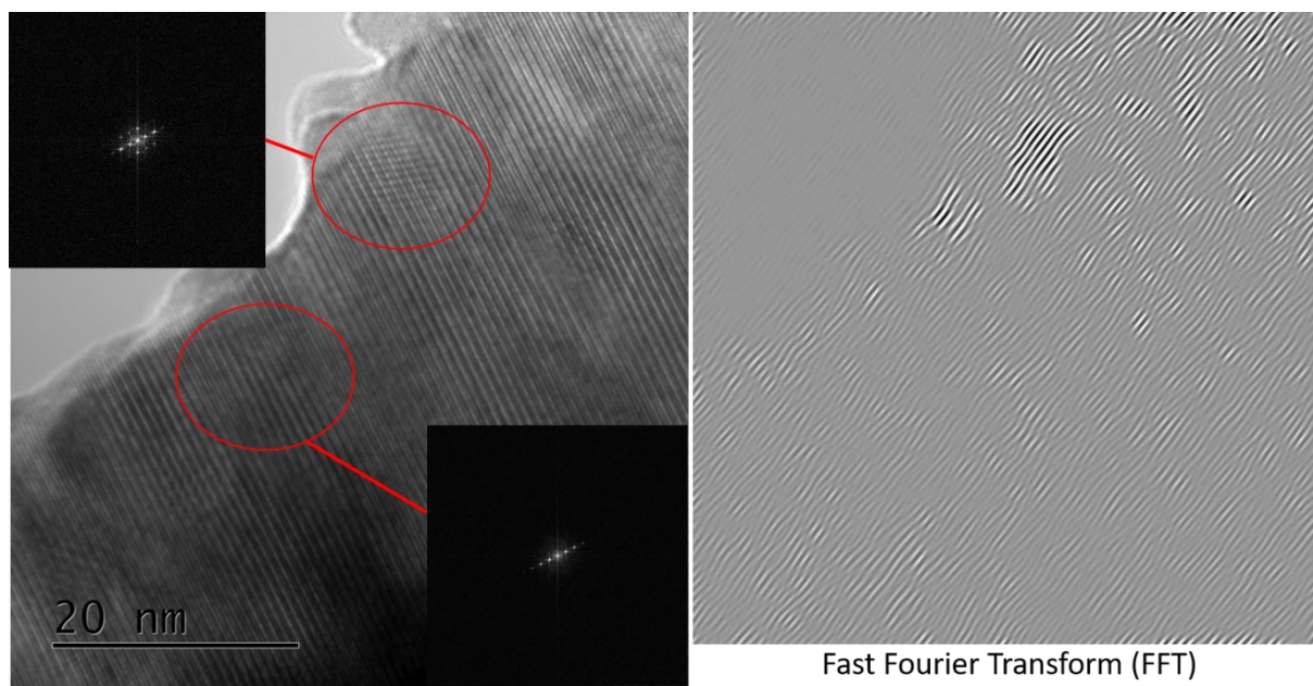
Figure 10: SAED and FFT images of BGLC 82, x = 0 , y = 0.2 .
