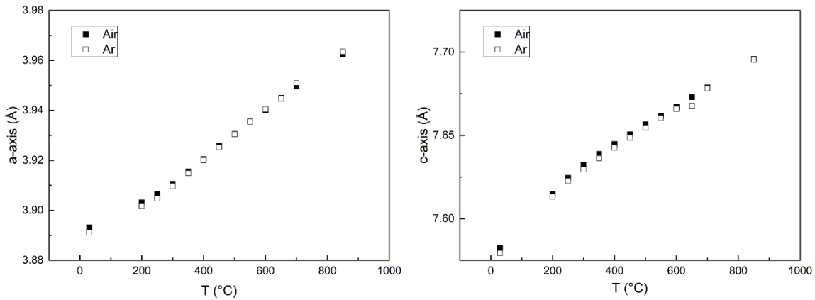
Figure 14: Cell parameters for a-axis (left) and c-axis (right) vs temperature for x = 0 in air (closed squares) and Ar (open squares) atmospheres.
