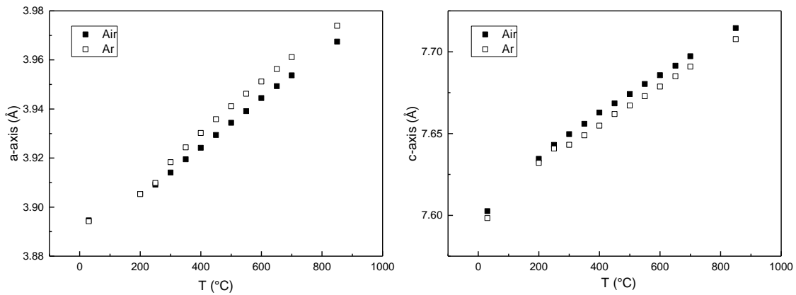
Figure 13: Cell parameters for a-axis (left) and c-axis (right) vs temperature for x = 0.1 in air (closed squares) and Ar (open squares) atmospheres.
