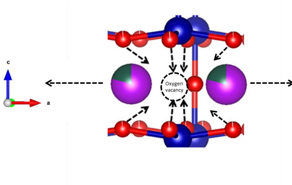
Figure 15: Coulombic forces around an oxygen vacancy in the Ln layer.
