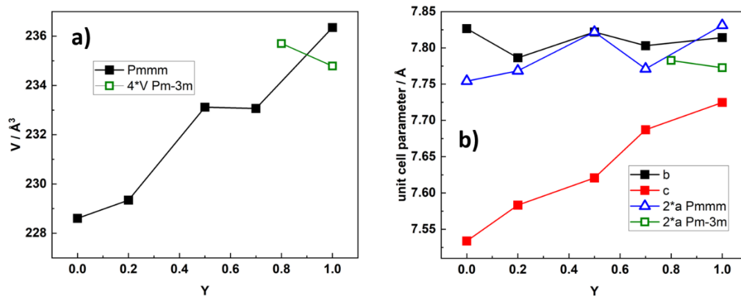
Figure 5: Unit cell volume (a) and cell parameters (b) for BGLC ( x = 0, y = 0-1 )
