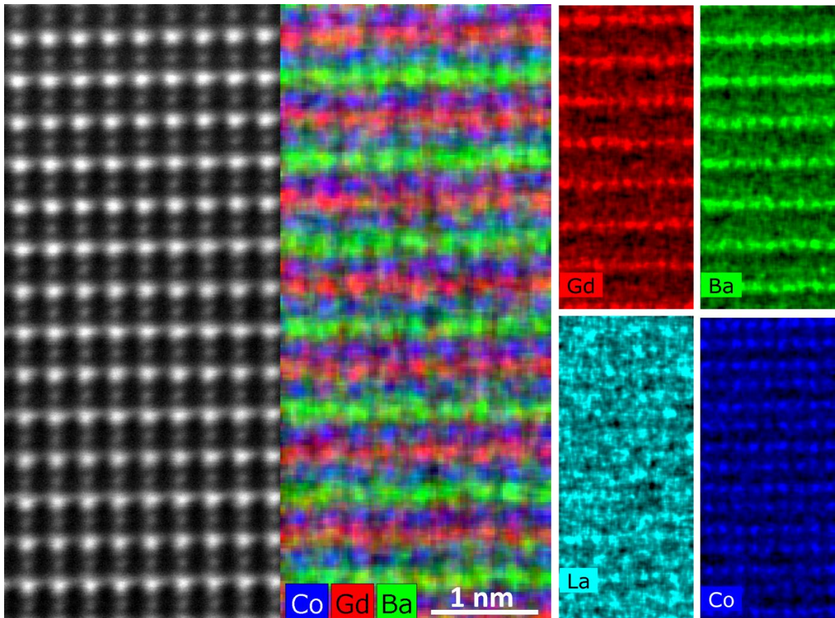
Figure 11: STEM Dark-Field image (left) and EDS elemental mapping (middle and right) of BGLC82 in dry state.
