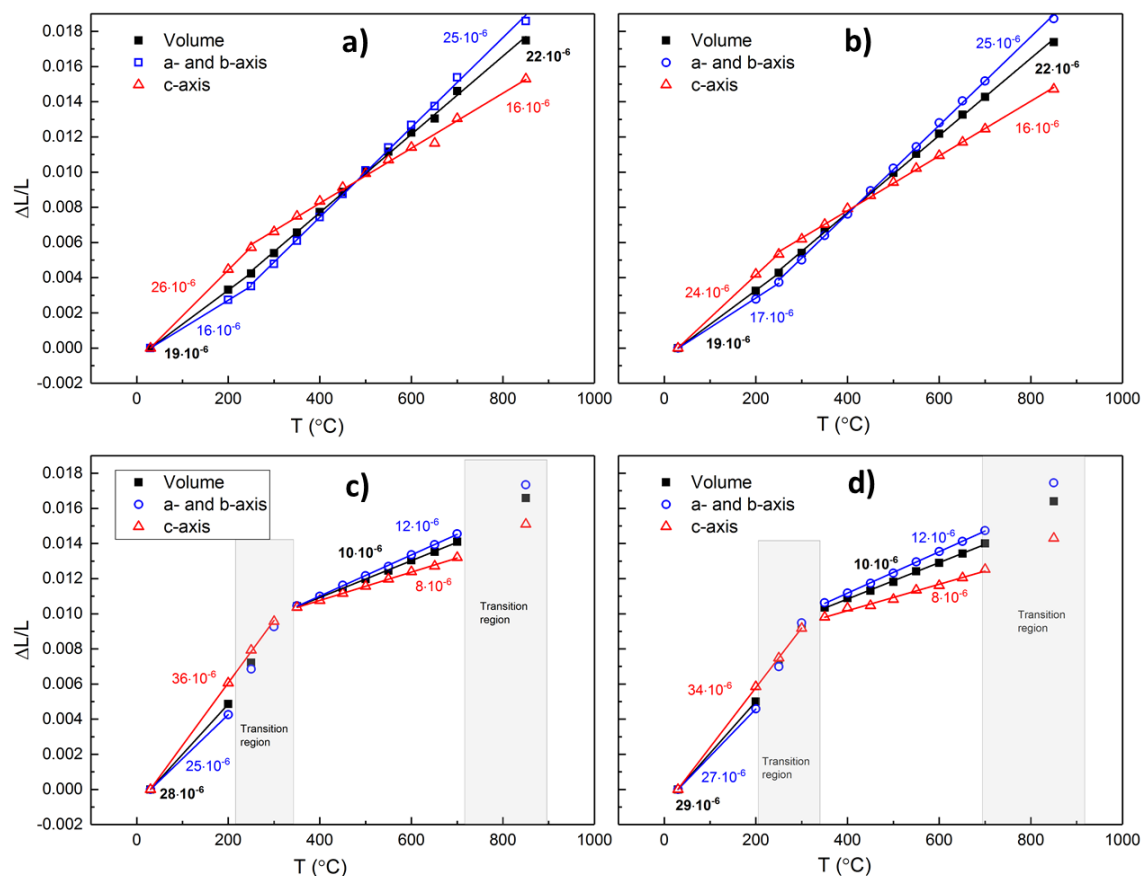
Figure 12: Thermal and chemical expansion of a- and b-axes and volume expansion in air for x = 0 (a), x = 0.1 (b), x = 0.2 (c) and 0.3 (d).
