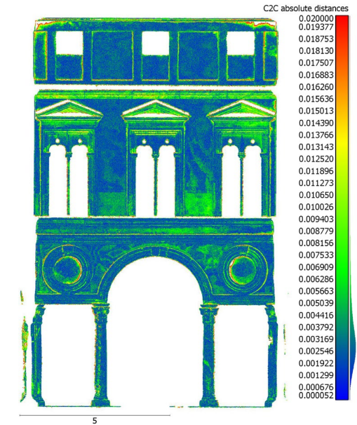
Fig. 14 - Point cloud comparison between the laser and the photogrammetric survey.
