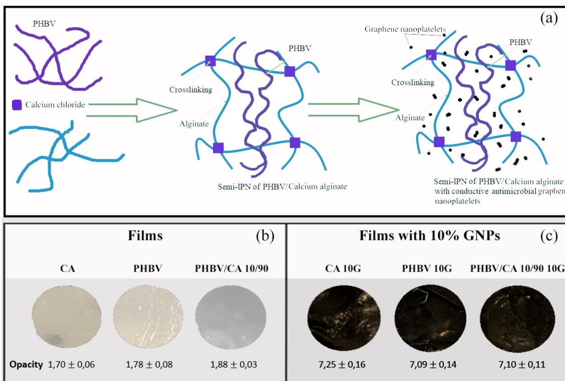
Figure 2. Schematic representation of the synthesis process (a) and the macroscopic morphology of the novel biodegradable semi-interpenetrated polymer network (semi-IPN) of poly(3-hydroxybutyrate-co-3-valerate) and crosslinked alginate (with calcium chloride) without (b) and with (c) conductive antimicrobial graphene nanoplatelets; 10G: 10% graphene nanoplatelets. The opacity of each film calculated by Eq. (1) is shown under each sample.
