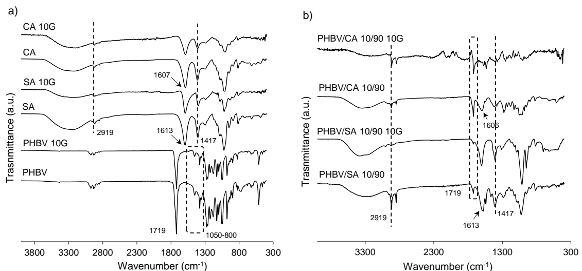
Figure 8. Fourier transform infrared spectroscopy (FTIR) spectra in the region 4000-300 \text{cm}^{-1} . a) Neat PHBV, SA and calcium alginate (CA), and samples with 10% of graphene nanoplatelets (10 G). b) PHBV/SA 10/90 blend, semi-IPN PHBV/CA 10/90, and nanocomposites with GNPs (10G). GNPs concentration: 10% w/w.
