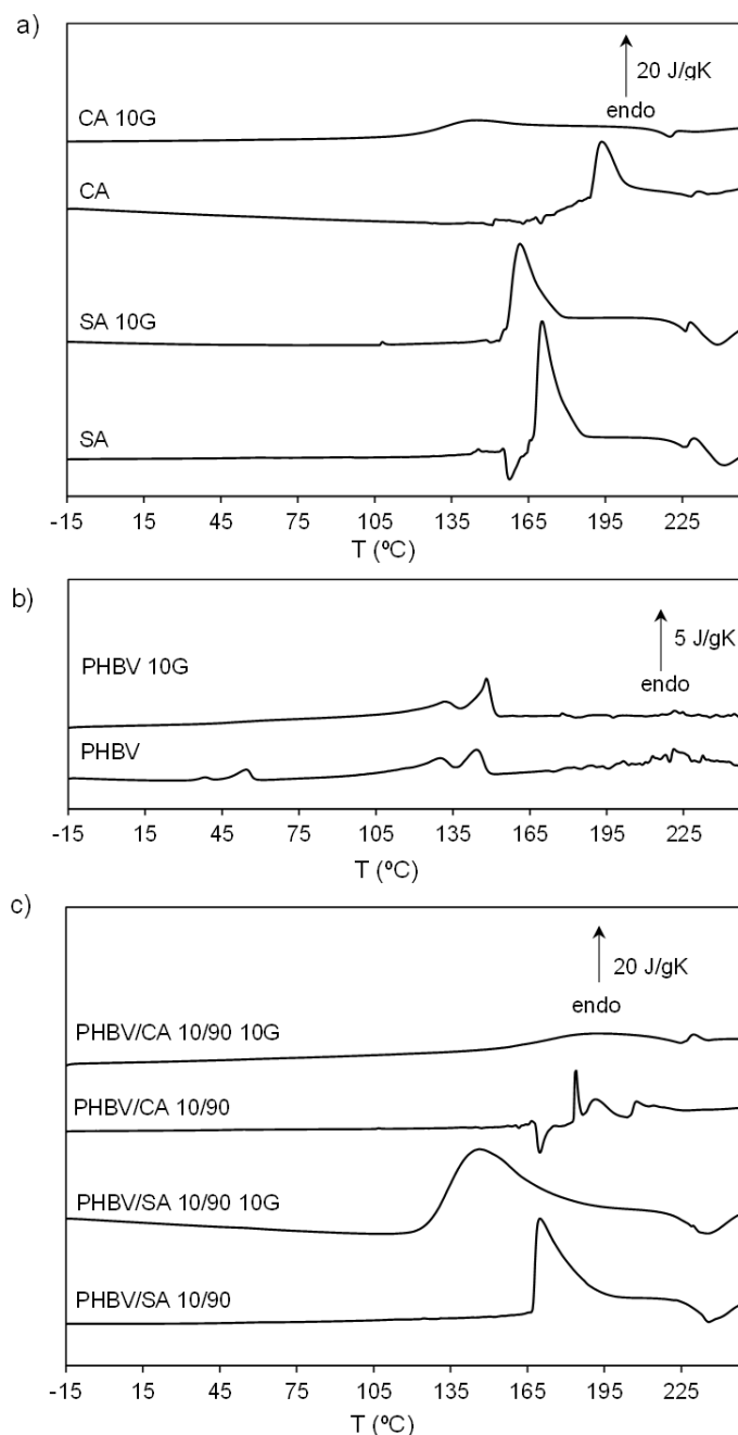
Figure 10. Differential scanning calorimetry (DSC) thermograms at a rate of 20 °C/min Normalized heat flow on heating. (a) Neat SA and crosslinked SA (CA) with and without GNPs (10G). (b) Neat PHBV with and without GNPs (10G). (c) PHBV/SA 10/90 blend, PHBV/CA 10/90 semi-IPN and nanocomposites with GNPs (10G). GNPs concentration: 10%.
