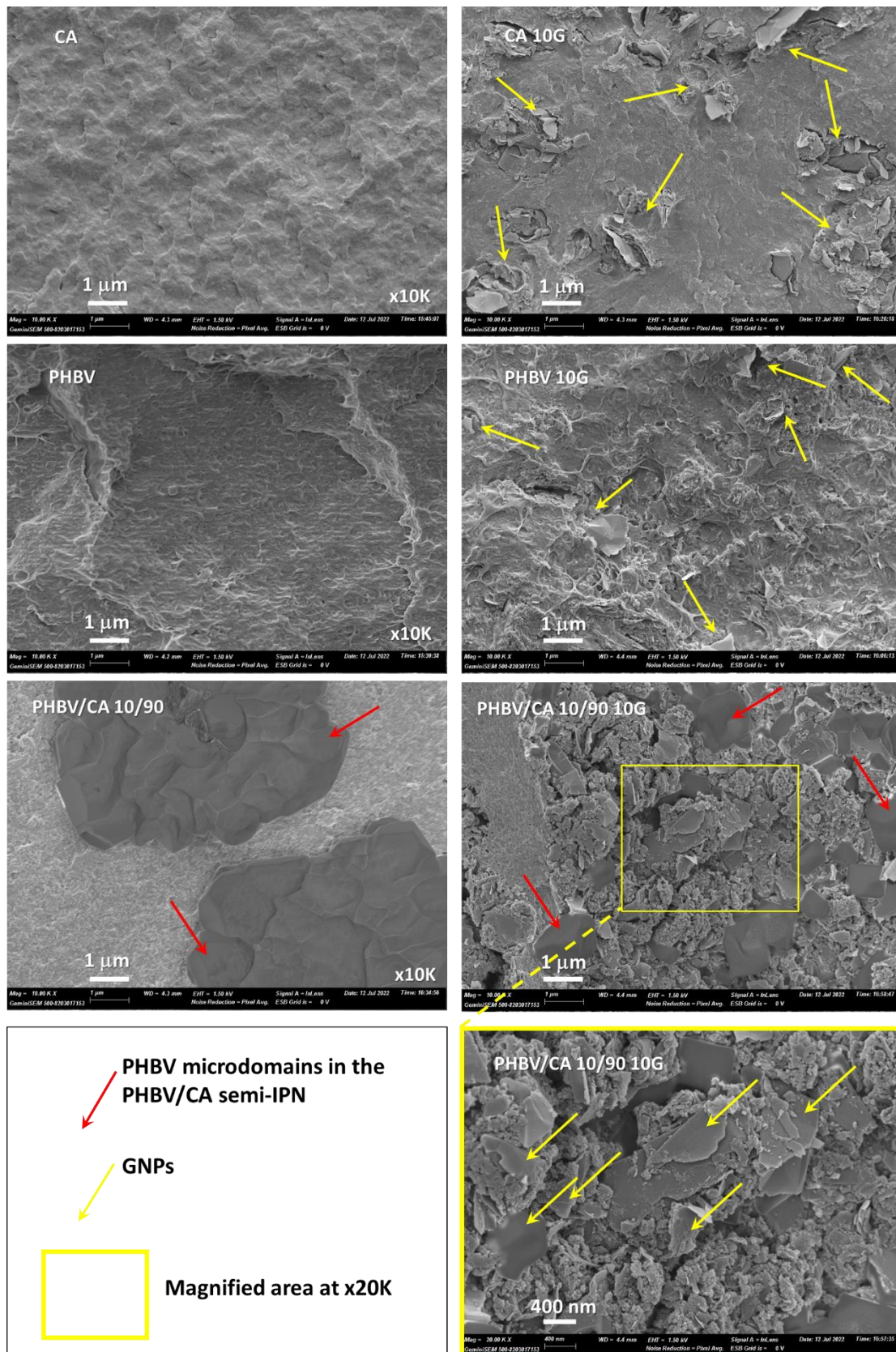
Figure 7. Material morphology: HR-FESEM observation after cryogenic fracture of the calcium alginate (CA), PHBV and semi-IPN PHBV/CA 10/90 sample films with and without 10% of GNPs (10 G) at x10000 and a magnified area at x20000. Yellow and red arrows indicate the GNPs present in the nanocomposites and microdomains of PHBV in the semi-IPN of the PHVA/CA 10/90 with and without 10% of GNPs, respectively.
