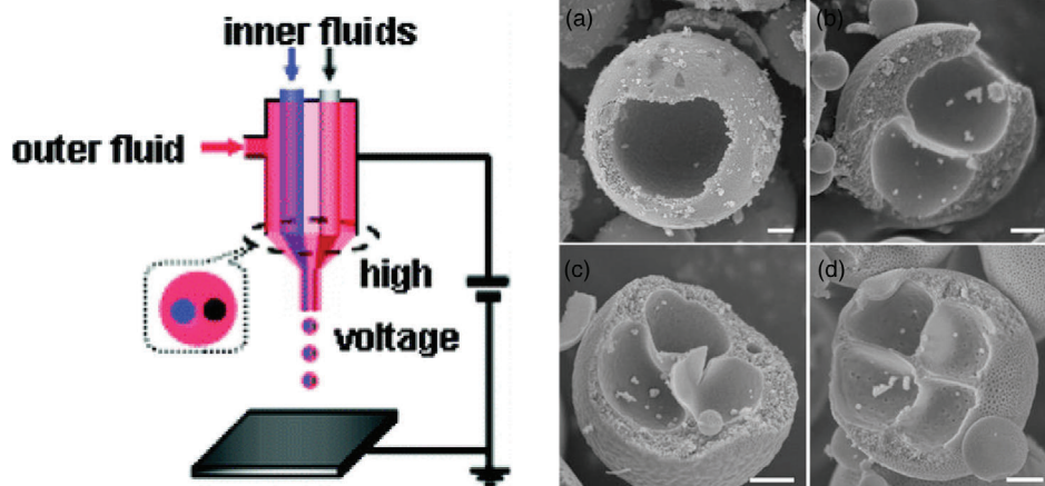
Figure 4. Experimental setup of compound-fluidic electrospraying (left) for the fabrication of microcapsules with several compartments (right). Reproduced with permission. [68] Copyright 2008, American Chemical Society.
