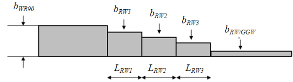
Fig. 12. Geometry and dimensions of the E -plane waveguide transformers (where the variable names are the ones used in Tables III and IV).
