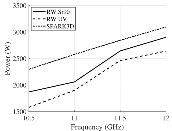
Fig. 21. Comparison of simulated (SPARK3D) and measured results, using Sr90 (RW Sr90) and UV light (RW UV) electron sources, of the transformer with an RW central section.
