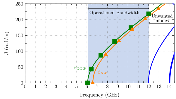
Fig. 2. Dispersion diagram of the GGW-90 (unwanted modes with solid lines and fundamental mode with square marks) and the WR-90 RW (fundamental mode with triangle marks).
