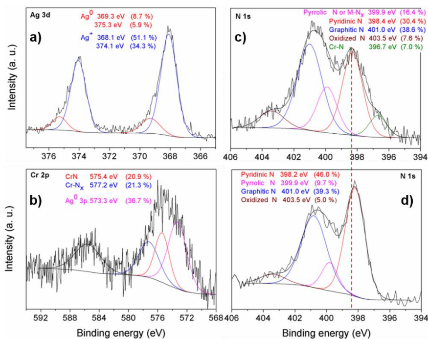
Figure 4. XPS spectra of Ag 3d (a), Cr 2p (b) and N 1s (c) core levels of catalyst \text{AgCr@CN-800} . (d) N 1s XPS spectrum of catalyst \text{M-free@CN-800} .
