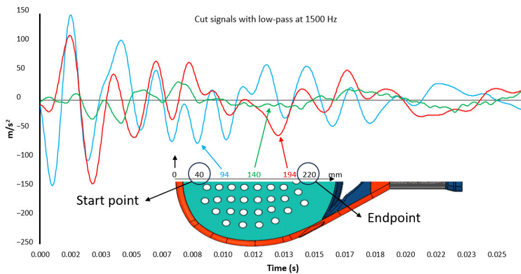
Figure 3. Example of accelerometer response when padel racket is hit at different points.
