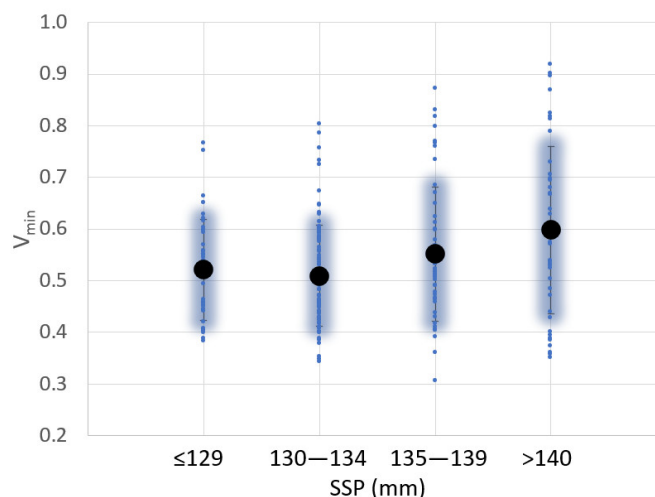
Figure 7. Variation of the sweet spot position (SSP) and V_{\min} value for 225 padel rackets analyzed.
