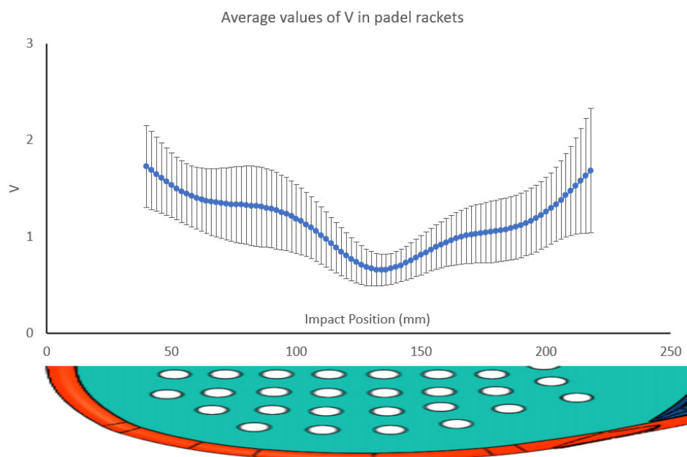
Figure 12. Variation of the V value for 225 padel rackets along its central line and standard deviation in every impact point.
