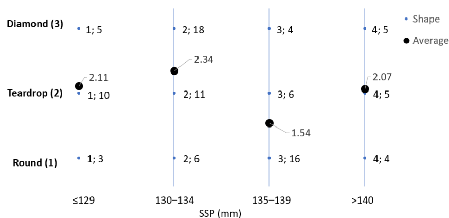
Figure 11. Variation of the sweet spot position (SSP) and padel racket shape for 93 padel rackets analyzed.
