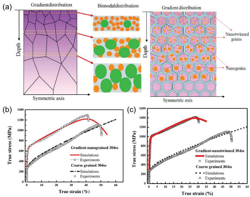
Fig. 14. Comparison between depth-dependent grain size and twin spacing structured 304 stainless steel (SS). (a) Representations of gradient structured (GS) 304 SS with depth-dependent grain size and twin density, as well as the comparison between the experimental and simulated stress-strain curves of (b) nano-grained GS and (c) nano-twinned GS 304 SS [535].
