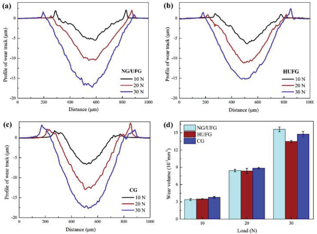
Fig. 23. Cross-sectional profiles of (a) nanograined/ultrafine grained (NG/UFG), (b) Heterogeneous UFG (HUFG) and (c) CG 18Cr-8Ni austenitic stainless steels (SS) under different loads, and (d) the wear volumes versus normal loads in three SS [630].
