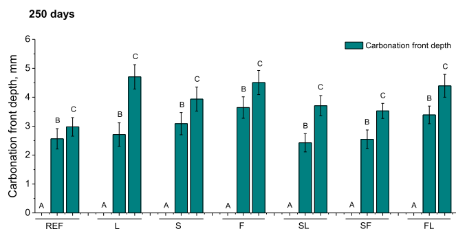
Fig. 6. Depths of carbonation front noted at 250 days.
