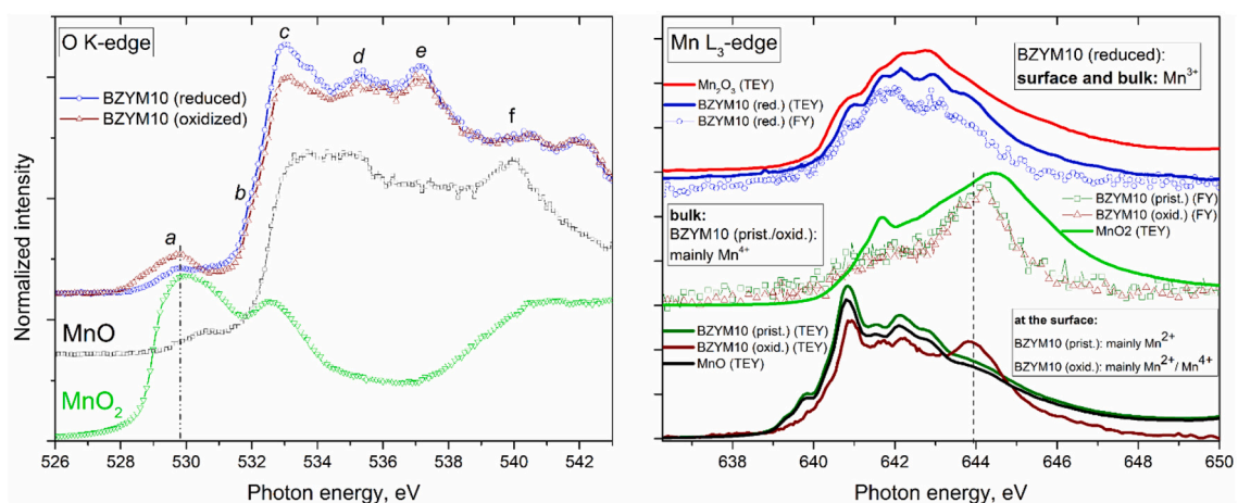
Fig. 13. Comparison of the NEXAFS spectra at O K-edge (left) and Mn L 3 -edge (right) of the studied compounds and some reference powders recorded in the TEY (solid line) and FY (symbols) modes.
