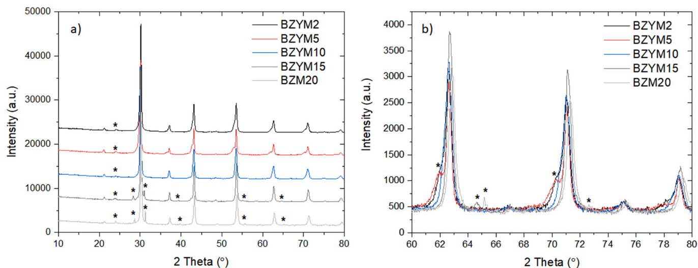
Fig. 2. XRD patterns of a) powder specimens of the series \text{BaZr}_{0.8}\text{Y}_{0.2-x}\text{Mn}_x\text{O}_{3.5} where x = 0.02; 0.05; 0.1; 0.15 and 0.20 (BZYM2, BZYM5, BZYM10, BZYM15, BZM20 respectively) after conventional solid state synthesis at 1400^\circ\text{C} for 6 h; b) Magnified XRD spectra excerpt in the 2\theta range of 60\text{--}80^\circ . Secondary phases are marked with an asterisk.
