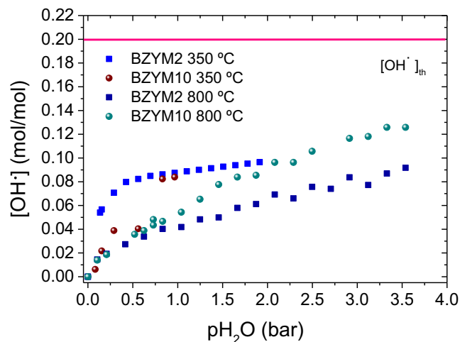
Fig. 10. a) Proton content registered for BZYM2 and BZYM10 as a function of p_{\text{H}_2\text{O}} at 350 °C and 800 °C; (pink line indicates the theoretical proton content according to the nominal stoichiometry). (For interpretation of the references to colour in this figure legend, the reader is referred to the web version of this article.)
