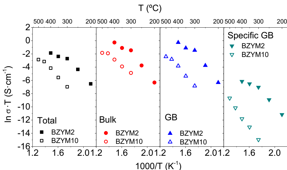
Fig. 11. EIS deconvoluted conductivity in humid (2.5 vol% H 2 O), 2 vol% H 2 /Ar of materials from the BaZr 0.8 Y 0.2-x Mn x O 3-s series, a) total, b) bulk, c) grain boundary (GB) and d) specific grain boundary, plotted as a function of the inverse temperature.
