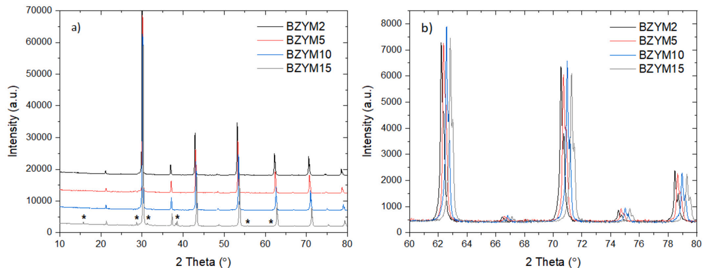
Fig. 3. XRD patterns of a) polished specimens of the series \text{BaZr}_{0.8}\text{Y}_{0.2-x}\text{Mn}_x\text{O}_{3.5} where x = 0.02; 0.05; 0.1 and 0.15 (BZYM2, BZYM5, BZYM10 and BZYM15, respectively) sintered at 1700^\circ\text{C} for 10 h; b) Magnified XRD spectra excerpt in the 2\theta range of 60\text{--}80^\circ : peaks shift to the higher 2\theta values with increasing the Mn content. Secondary phases are marked with an asterisk.
