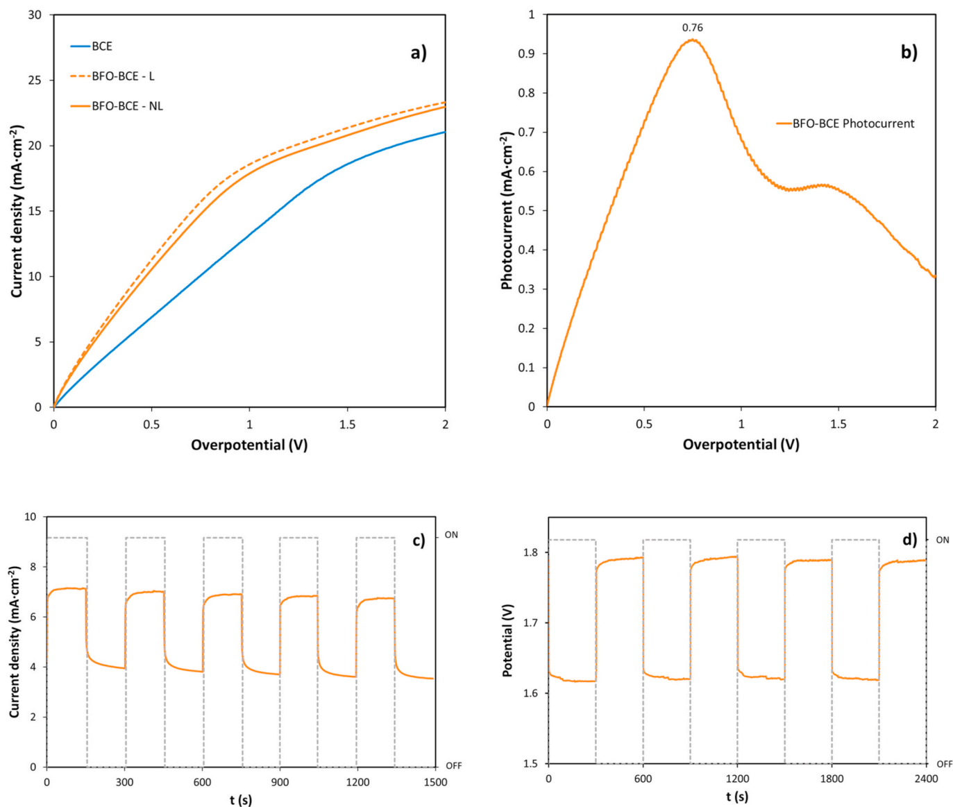
Fig. 2. (a) LSV of the BFO-BCE and BCE anodes in a 0.1 M \text{Na}_2\text{SO}_4 solution in presence (L) and absence (NL) of light (b) BFO-BCE photocurrent evolution under light effect. (c) Chronoamperometry using light pulses for the BFO-BCE electrodes, applying an overpotential of 0.5 V. (d) Chronopotentiometry using light pulses for the BFO-BCE electrode, applying 5.2 \text{mA cm}^{-2} .
