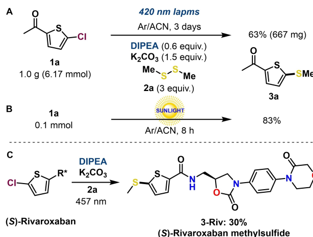
Scheme 6. A: Upscaling of the model reaction. B: Use of sunlight irradiation. C: Application of a late stage thiolation. See the Supporting Information for detailed information.
