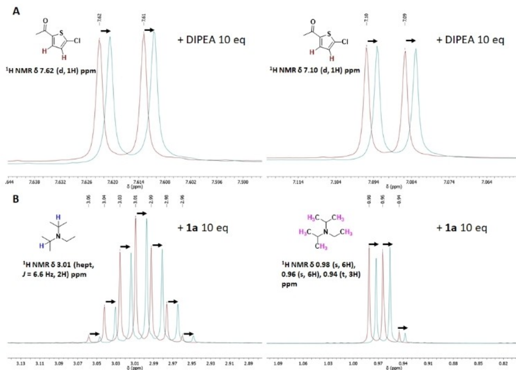
Figure 1. A: Relevant part of the ^1\text{H} NMR spectra of the starting material 1a (0.033 M) in the absence (red) and in the presence of 10 equiv. of DIPEA (green). B: Relevant part of the ^1\text{H} NMR spectrum of DIPEA (0.033 M) in the absence (red) and in the presence of 10 equiv. of 1a (green). Measurements were carried out in deuterated acetonitrile \text{CD}_3\text{CN} .
