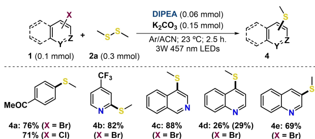
Scheme 5. Reaction scope of 6-membered (hetero)arene halides and dimethyl disulfide through EDA complexes. Full conversion of starting materials 1 in all cases unless otherwise indicated in brackets. For detailed information on the reaction conditions, see the Supporting Information.
