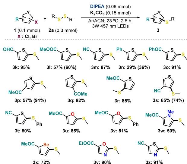
Scheme 4. Reaction scope of 5-membered heteroarene halides 1 through EDA complexes. Full conversion of starting materials 1 in all cases unless otherwise indicated in brackets. For detailed information on the reaction conditions, see the Supporting Information.
