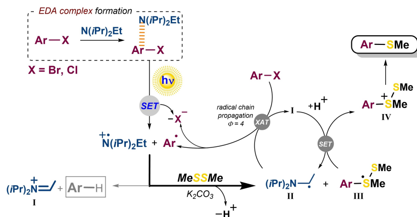
Scheme 2. Visible-light-powered thiolation of heteroarenes through EDA complexes.
