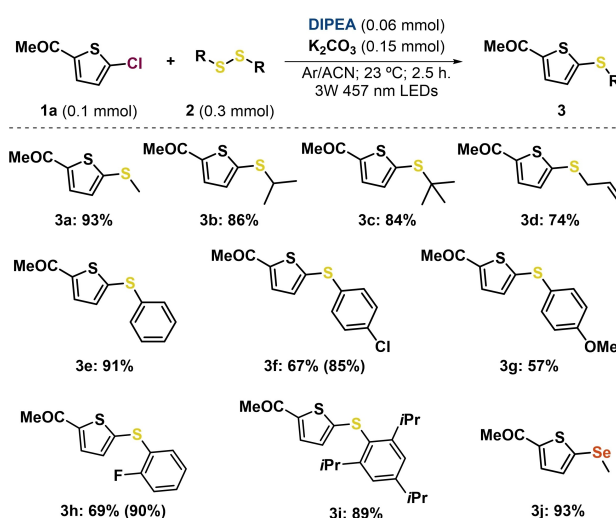
Scheme 3. Reaction scope of 1a and disulfide derivatives through EDA complexes. Full conversion of compound 1a in all cases unless otherwise indicated in brackets. For detailed information on the reaction conditions, see the Supporting Information.
