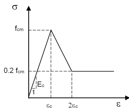
Figure 5. HSC constitutive model.
