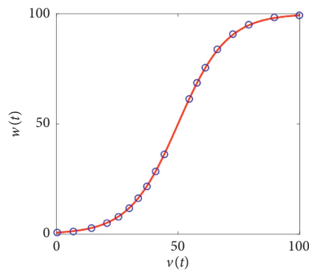
FIGURE 18: Example 3: comparison between real nonlinear function tansig (red) and captured nonlinearity (blue circles).
