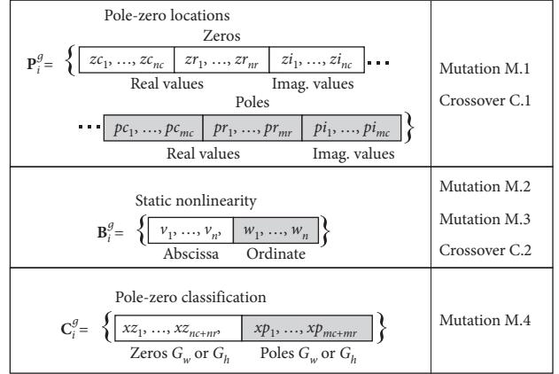
FIGURE 7: Structure of an individual and genetic operations performed on each piece of genetic information.
