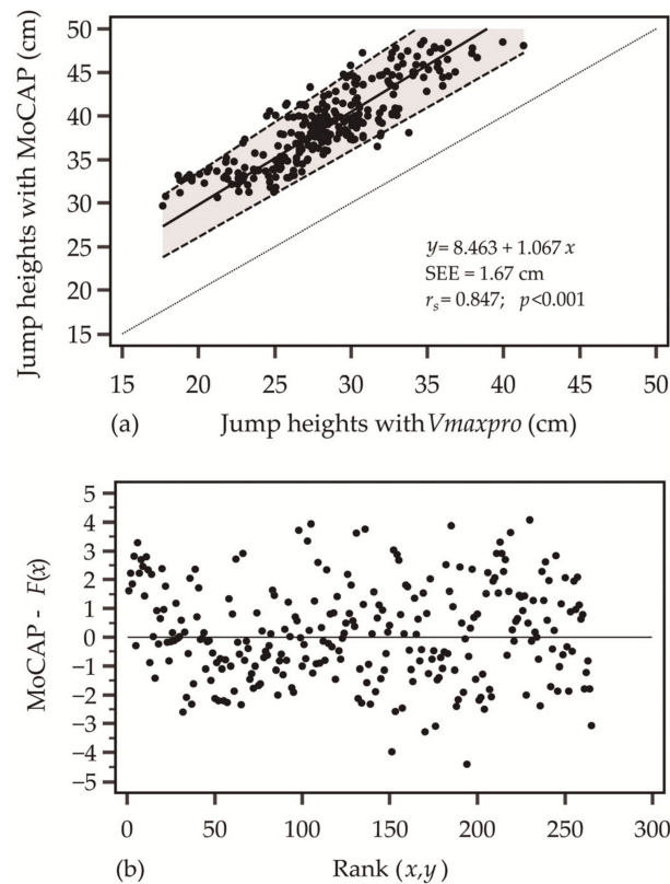
Figure 2. Correlation analysis between MoCAP system and Vmaxpro IMU through Passing and Bablok regression (a): the continuous line represents the regression line; the shaded area represents the confidence intervals for 95% of the regression line; the grey line is the x = y line; r_s represents Spearman's correlation coefficient; SEE standard error of the estimate. (b) Residuals plot: No trend is shown, so linearity is assumed.
