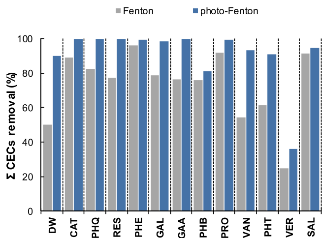
Fig. 8. \Sigma CECs removal (%) at t = 15 \text{ min} in Fenton and photo-Fenton process in the presence of selected ligands tested as auxiliaries in this study. Experimental conditions: [\text{Fe}(\text{II})] = 0.09 \text{ mmol}\cdot\text{L}^{-1} , [\text{Ligand}] = 0.227 \text{ mmol}\cdot\text{L}^{-1} , \text{pH} = 5 . Results in the absence of ligand are also given (labelled as DW).
