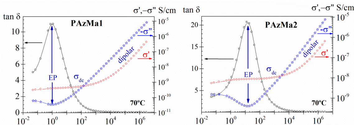
Figure 9. Frequency dependence of \tan \delta and of the real ( \sigma' ) and imaginary ( -\sigma'' ) parts of the complex conductivity ( \sigma^* ) for PAzMa1 and PAzMa2 at 70\text{ }^{\circ}\text{C} .
