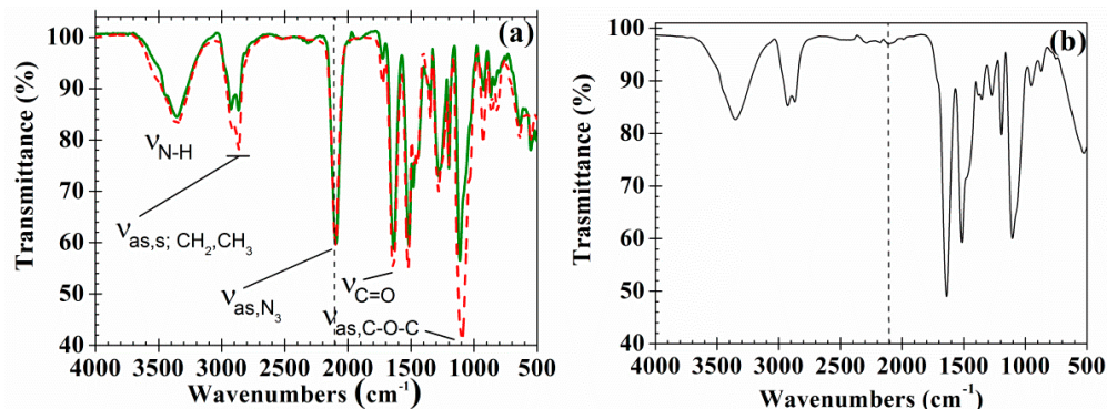
Figure 3. (a) Normalized ( \nu_{as,N_3} peak) FTIR spectra of PAzMa1 (continuous line) and PAzMa2 (dash dot line) films and (b) FTIR spectra of PAzMa1 after thermal treatment (heated in TGA from rt to 250 °C at 1 °C·min -1 ).
