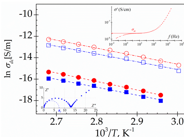
Figure 14. Temperature dependence of the dc conductivity (S/m) for PAzMa1 (full symbols) and PAzMa2 (open symbols) evaluated from the plateau at low temperatures of \sigma' versus f (circles) and from the Cole-Cole impedance plots (squares).
