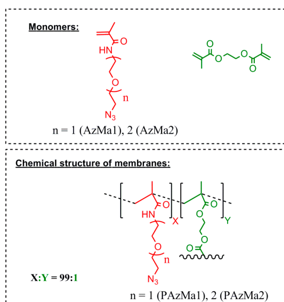
Figure 1. Chemical structure of films, PAzMa1 and PAzMa2 and monomers used in their preparation.
