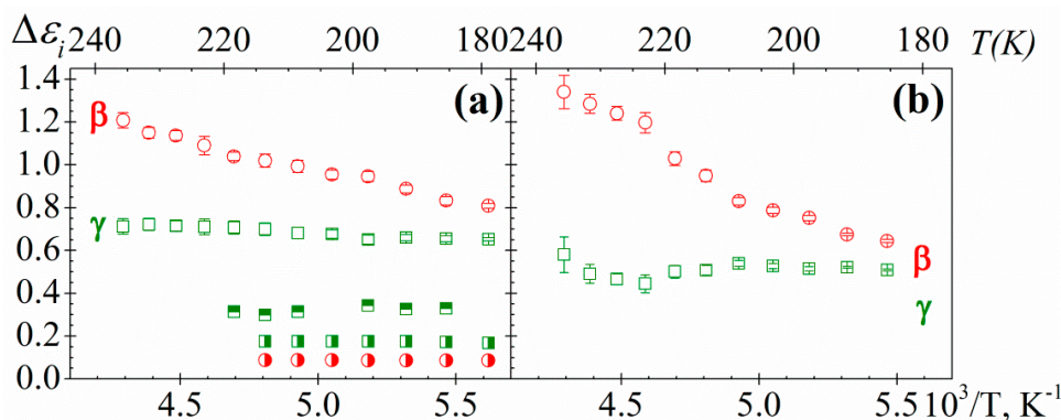
Figure 11. Temperature dependence of the strength for \gamma (squares) and \beta (circles) relaxations of (a) PAzMa1 and (b) PAzMa2 samples. In (a) has been shown the strength relaxation values corresponding to the PEOEMA (square with right half black, circle with right half black) and CEOEMA (square with top half black) samples [9].
