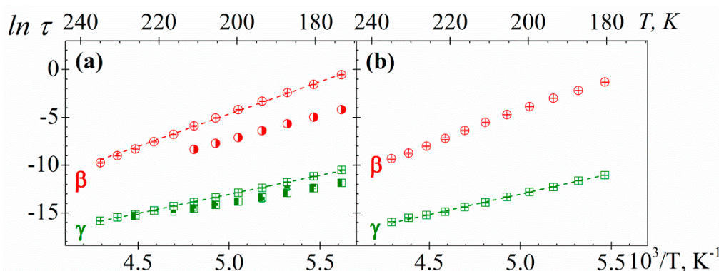
Figure 12. Arrhenius plot for \gamma (squares) and \beta (circles) relaxations of (a) PAzMa1 and (b) PAzMa2 samples. In (a) has been shown the time relaxation values corresponding to the PEOEMA (square with right half black, circle with right half black) and CEOEMA (square with top half black) samples [9].
