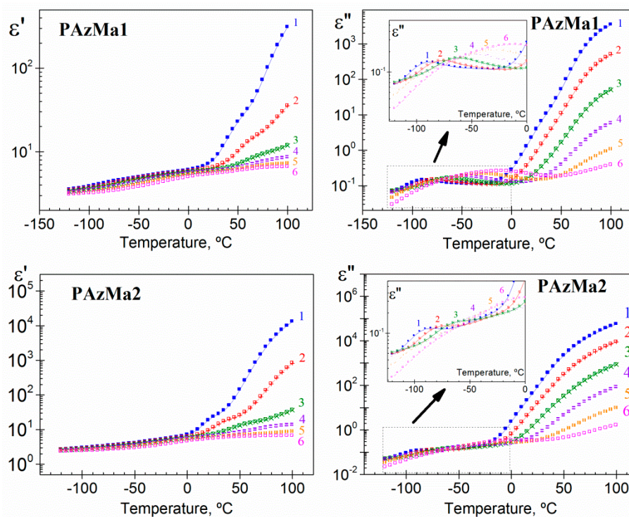
Figure 6. Real and loss components of the complex dielectric permittivity as a function of temperature for PAzMa1 and PAzMa2 at 1.19 \times 10^0 [1: square], 8.73 \times 10^0 [2: ballot box with +], 9.52 \times 10^1 [3: ballot box with ×], 1.04 \times 10^3 [4: square with top half black], 1.13 \times 10^4 [5: square with right half black] and 1.2 \times 10^5 [6: square containing black central point].
