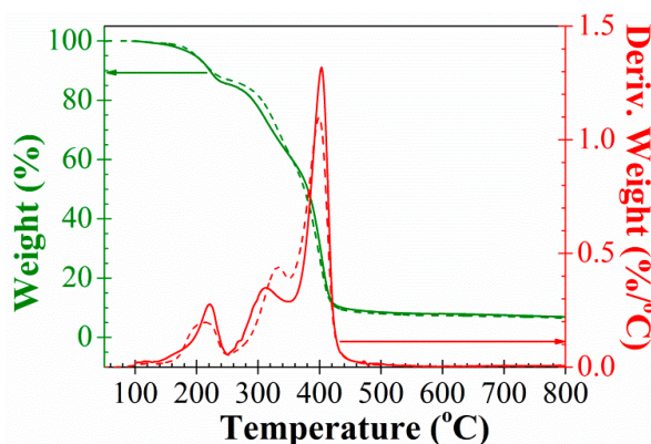
Figure 4. TGA and first derivative TGA curves of PAzMa1 (continuous line) and PAzMa2 (short dot line) samples.
