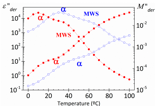
Figure 7. Temperature dependence of the loss permittivity (square) and loss modulus (circle) derivative spectra of the PAzMA1 (open symbols) and PAzMA2 (full symbols) at 1.19 \times 10^0 Hz.
