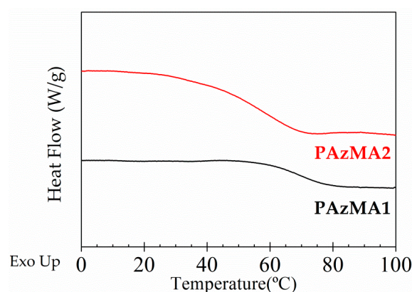
Figure 5. DSC experimental curves for PAzMa1 (bottom) and PAzMa2 (above) samples.
