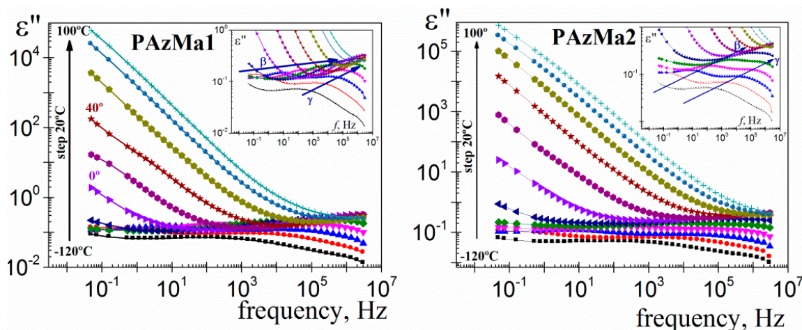
Figure 8. Dielectric loss permittivity as a function of frequency for PAzMa1 and PAzMa2 in the temperature range -120\text{ }^{\circ}\text{C} – 100\text{ }^{\circ}\text{C} (at 20\text{ }^{\circ}\text{C} steps).
