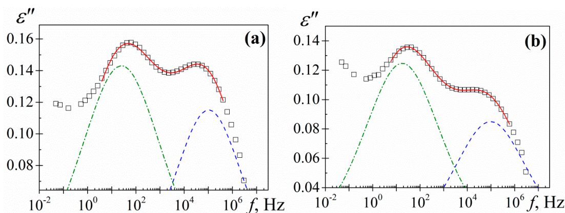
Figure 10. Deconvolution of loss factor for (a) PAzMa1 and (b) PAzMa2 at -70^\circ\text{C} . Squares represent the experimental data, continuous line the HN fitting curve and dashed lines the individual processes.
