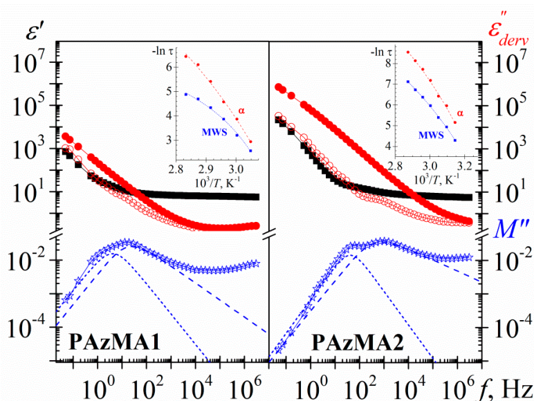
Figure 13. Frequency dependence of the dielectric constant (square), experimental loss permittivity (full circle), derivative loss permittivity (open circle) and derivative loss modulus (star) spectra of the PAzMA samples at 60 °C. Short dashed lines correspond to the MWS process and dashed lines to the \alpha relaxation process. Inset: Temperature dependence of the relaxation time in the Arrhenius coordinates.
