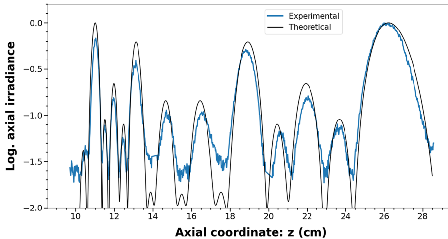
Fig. 5 Comparison of numerical and experimental axial irradiance of a SMZP of order 5
