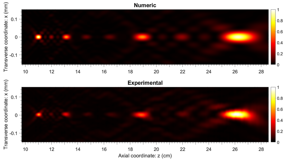
Fig. 6 Evolution of the transverse intensity distribution produced by a SMZP of order 5
