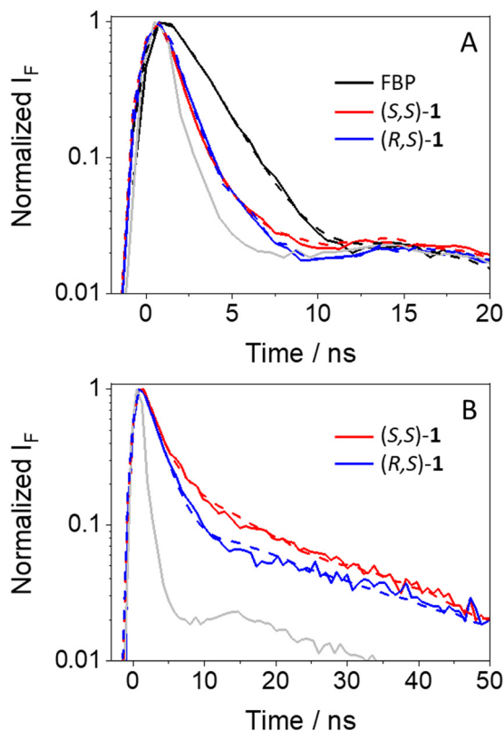
Fig. 4 Decay traces at the maximum emission (A) and at wavelengths longer than 420 nm (B) for ( S )-FBP (black), ( S,S )-1 (red) and ( R,S )-1 (blue) after excitation at 265 nm in acetonitrile. The best fitting curves are shown in dashed. The instrumental response function is shown in light gray.
