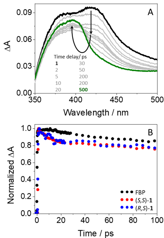
Fig. 5 (A) Femtosecond transient absorption spectra for ( S,S )- 1 from 1 ps (black) to 0.5 ns (green). (B) Kinetic traces for ( S )-FBP (black), ( S,S )- 1 (red) and ( R,S )- 1 (blue) at 425 nm. All measurements were performed upon excitation at 250 nm in acetonitrile.
