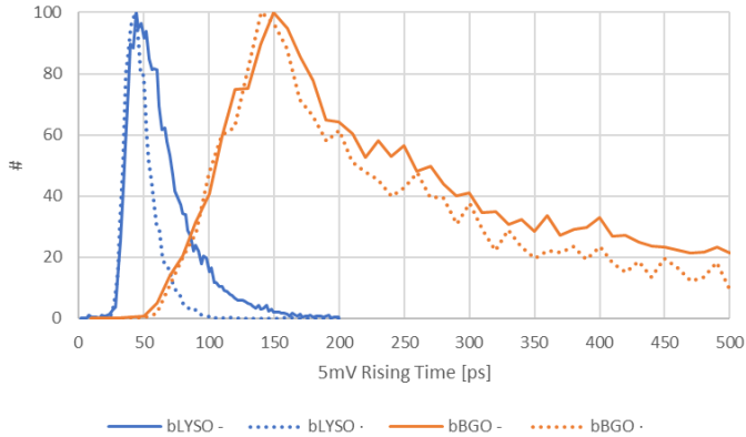
Figure 8. Comparison RTD plots of bLYSO (in blue) and bBGO (orange) choosing cFS events (solid lines) and cPP events (dotted lines). In both cases the sensor used is a NUV-HD coupled with SS.
