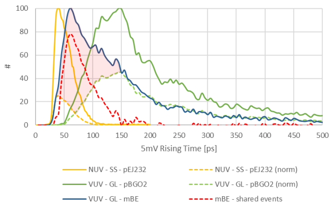
Figure 11. RTD distributions of pEJ232 events coupled with SS to NUV-HD sensor (yellow line), and pBGO2 and mBE coupled with glycerin to VUV-HD sensor (respectively, green, and blue lines). The solid lines are normalized by the maximum value of the relative distributions, while the yellow and green dashed ones are a normalized version of those with the same color. Last, the dashed red line shows the projection of the red area containing only the shared mBE events.
