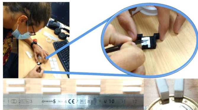
Figure 3. (Top) Metapixel manufacturing process. (Bottom-left) Some of the metapixels in our disposal. (Bottom-right) Metapixel cross-section with the two compound materials clearly distinguishable.
