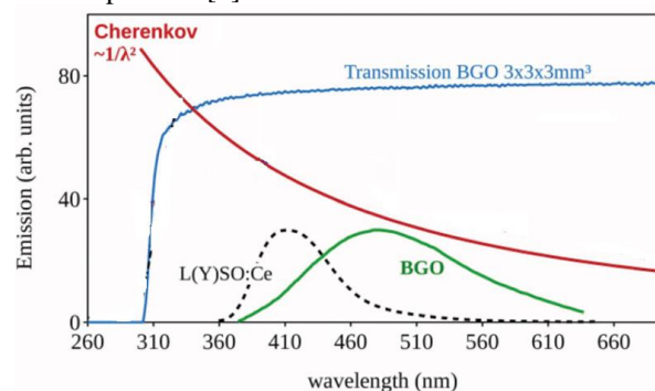
Figure 1. Emission spectra of BGO, LYSO:Ce and Cherenkov radiation compared to the BGO transmission. Modified from [5].
