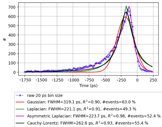
Figure 7. Asymmetric distribution using bLYSO as reference detector and bBGO as tester with different fitting results. The maximum of the distribution is around -180 ps.
