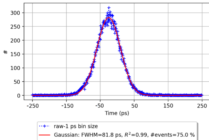
Figure 9. CTR result of two bLYSO coupled with SS-988 to NUV-HD sensors.
