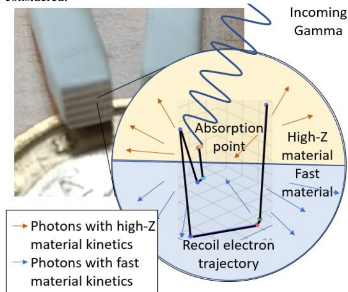
Figure 2. Recoil trajectory and photon generation inside a metapixel [10].
