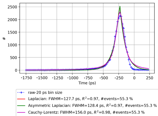
Figure 15. CTR result of mBE couple with glycerin to a VUV-HD sensors and filtering just those events that are faster than 100 ps of the RTD distribution.
