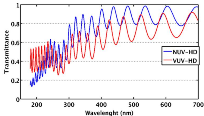
Figure 4. Calculated transmittance in silicon of normal incident light on the near ultraviolet high-density antireflective coating (NUV-HD ARC, blue line) and on the modified ARC of VUV-HD SiPMs. Taken from [15].
