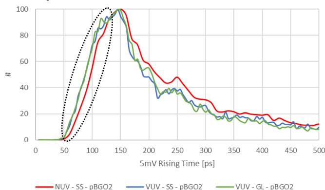
Figure 13. RTD distributions of pBGO2 cPP events coupled with SS-988 and glycerin to NUV-HD and VUV-HD sensors. Highlighted in the black dotted oval, the difference in Cherenkov population between NUV-HD and VUV-HD
