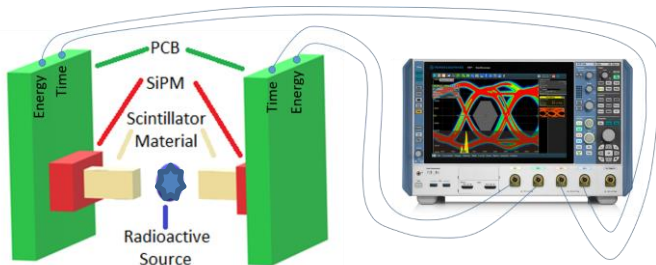
Figure 6. Coincidence HF Setup's sketch.
