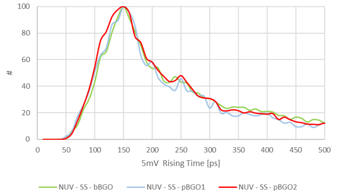
Figure 10. RTD distributions of cPP events of bBGO, pBGO1 and pBGO2 coupled with SS-988 to NUV-HD sensors.
