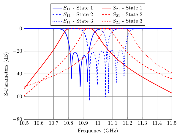
FIGURE 11. Electrical response of the HA filter.
