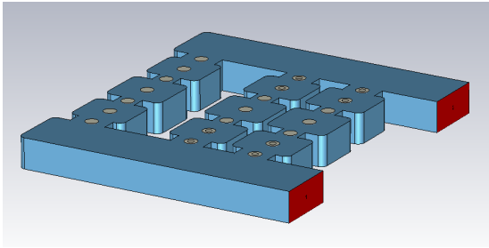
FIGURE 1. Reconfigurable rectangular waveguide filter structure for high-power applications.
