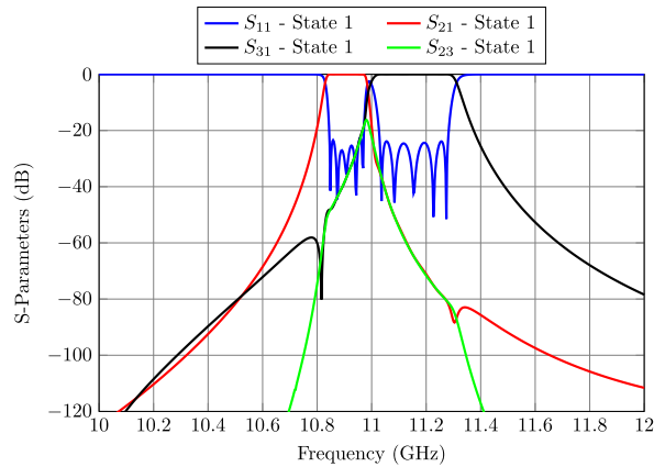
FIGURE 32. LA models for the first (top) and second (bottom) states of the designed diplexer.
