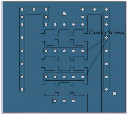
FIGURE 13. Closing screws of Filter B.
