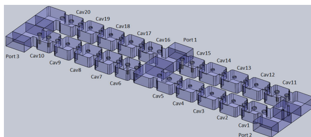
FIGURE 41. Structure for the state 1 of the reconfigurable diplexer.
