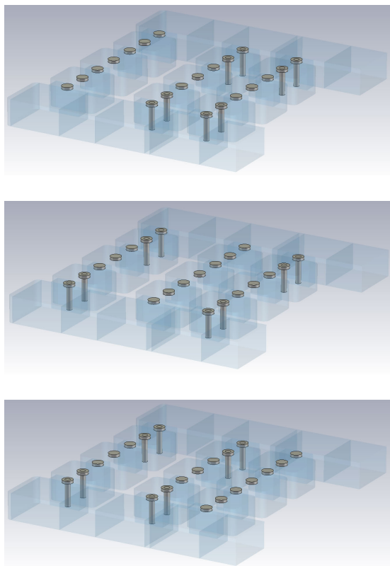
FIGURE 3. MTP configurations for selecting the different states: first (top), second (central) and third states (bottom).
