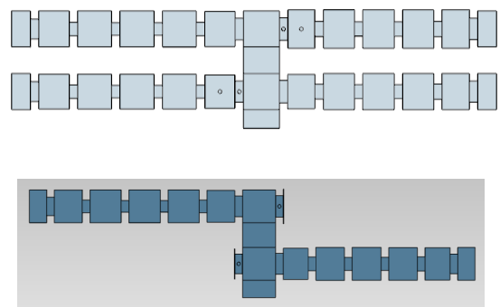
FIGURE 23. The isolated filters are combined considering the whole diplexer (top) or a reduced structure (bottom).
