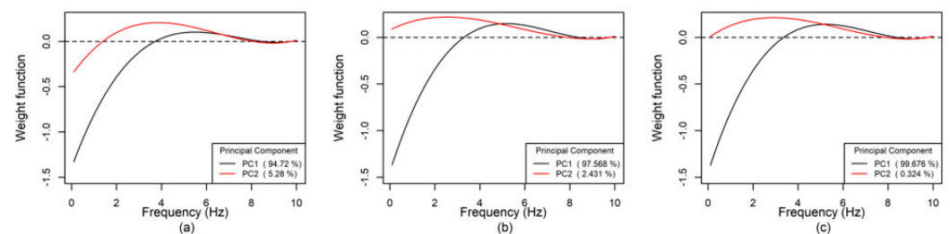
Figure 5. Weight functions for PC1 and PC2, obtained from functional analysis for (a) storage modulus G' , (b) loss modulus G'' , and (c) complex viscosity \eta^* .
