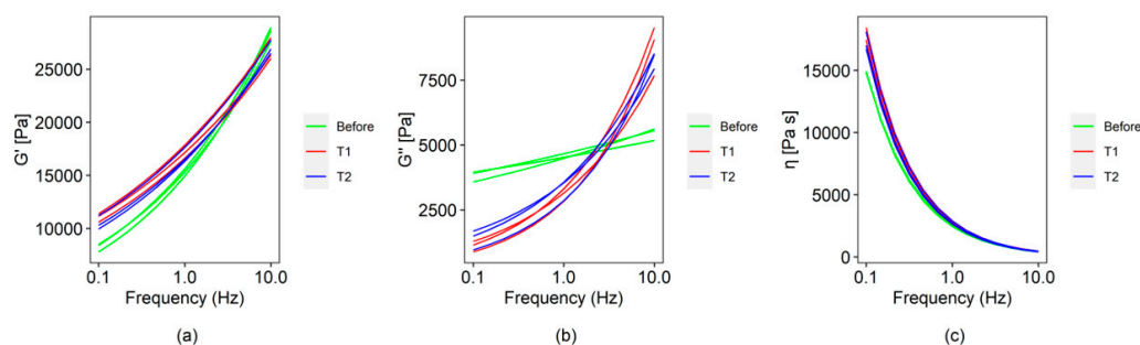
Figure 2. Rheological parameters curves for rice protein before (green line) and after printing (T1 = red line and T2 = blue line): (a) storage modulus [ G' ], (b) loss modulus [ G'' ], and (c) complex viscosity [ \eta^* ]. T1 (printing speed = 35 mm/s, layer height = 1.5 mm, nozzle diameter = 1.7 mm) and T2 (printing speed = 50 mm/s, layer height = 1 mm, nozzle diameter = 1.2 mm).
