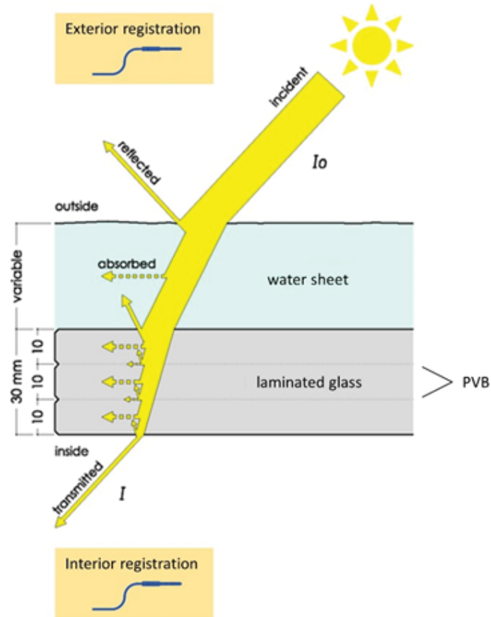
Figure 2. Light intensity attenuation through the skylight the skylight and the water layer. The initial intensity is represented by " I_o " so that it is reduced by the partial absorption and reflection that occurs circulating through the different layers, reaching the transmission of a fraction to the interior " I ".
