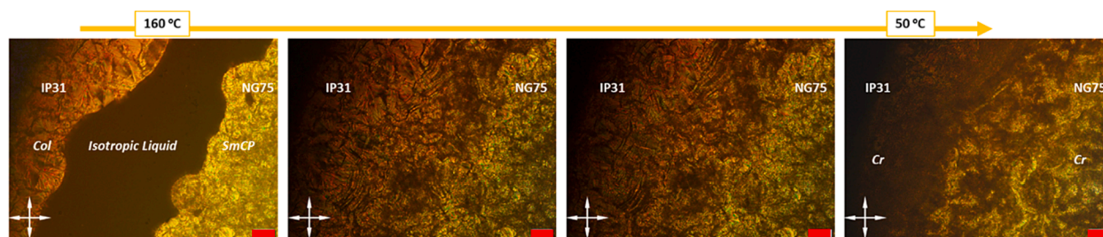
Fig. 2. Optical textures between crossed polarizers of a contact preparation of IP31-AzB and NG75-COO between two glass plates, uncoated cells, in a cooling process at 10\text{ }^{\circ}\text{C}\cdot\text{min}^{-1} from isotropic liquid phases. Red scale equals 50 \mu\text{m} .
