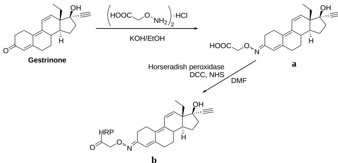
Figure 3. Synthesis of gestrinone oxime hapten (a) and gestrinone oxime hapten-horseradish peroxidase (HRP) conjugate (b).
