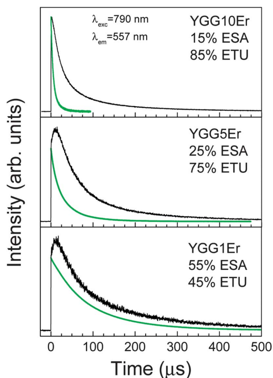
Fig. 10 Temporal evolution of the green upconverted luminescence of the \text{Er}^{3+} ions in YGG1Er, YGG5Er and YGG10Er nano-garnets after a 790 nm laser pulsed excitation. The luminescence decay curves of the green emission under direct excitation of the ^2\text{H}_{11/2} and ^4\text{S}_{3/2} multiplets at 525 nm are also included for comparison.
