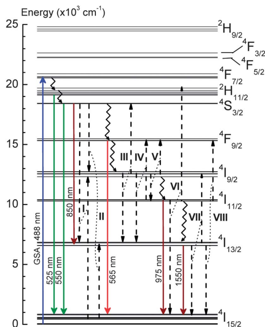
Fig. 5 Partial energy level diagram of the \text{Er}^{3+} ion showing different radiative transitions (downward solid lines) related to the luminescence after a ^4I_{15/2} \rightarrow ^4F_{7/2} ground state absorption (GSA) under a direct laser excitation at 488 nm. The multiphonon (zig-zag lines) and energy transfer (dashed lines) non-radiative relaxation processes are also shown.
