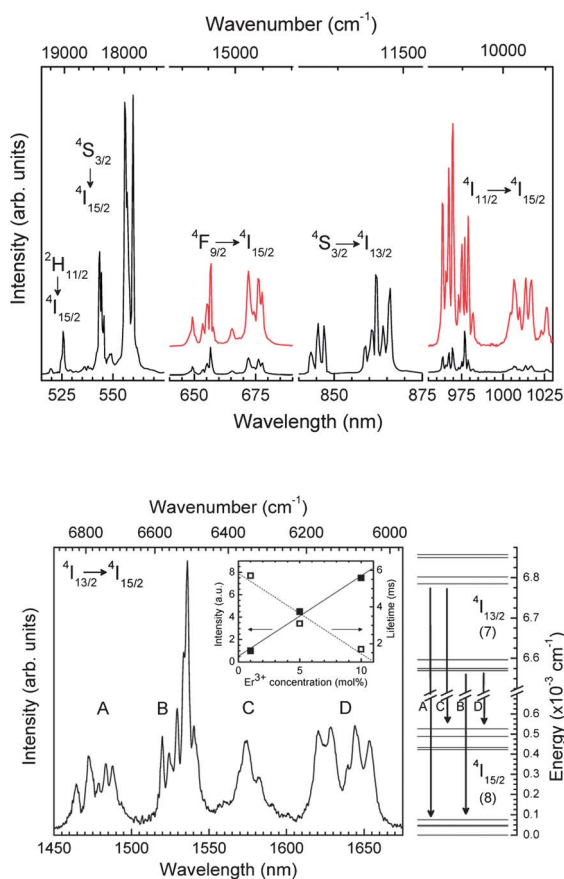
Fig. 6 (Top) Luminescence spectra of the YGG1Er and YGG10Er (overimposed) nano-garnets in the visible-NIR range at RT. The spectra are normalized to the intensity of the {}^2\text{H}_{11/2}, {}^4\text{S}_{3/2} \rightarrow {}^4\text{I}_{15/2} green emission. (Bottom) 1.5 \mu\text{m} {}^4\text{I}_{13/2} \rightarrow {}^4\text{I}_{15/2} NIR luminescence of the YGG1Er nano-garnet. The different bands are correlated to transitions between the {}^4\text{I}_{13/2} and {}^4\text{I}_{15/2} Stark levels. The degeneracies of the ground and the first excited multiplets are given in parenthesis. The inset figure shows the relative intensities of the {}^4\text{I}_{13/2} \rightarrow {}^4\text{I}_{15/2} emission and the lifetime of the {}^4\text{I}_{13/2} level as a function of the \text{Er}^{3+} concentration.
