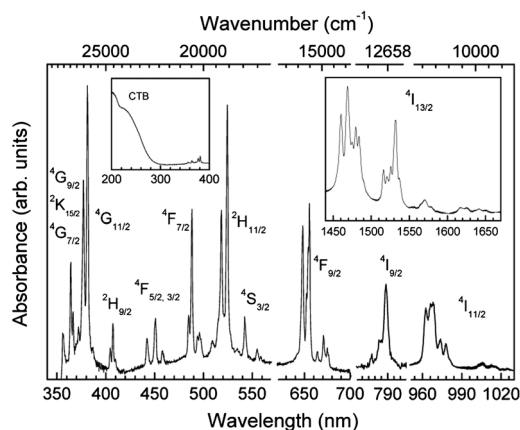
Fig. 4 Diffuse reflectance spectrum of the YGG5Er nano-garnet powder in the UV-visible-NIR range at RT. All transitions start from the ^4I_{15/2} ground state to the indicated levels.
