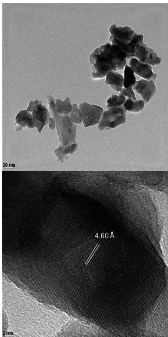
Fig. 1 High resolution transmission electron microscope (HRTEM) micrographs of the YGG nano-garnets.
