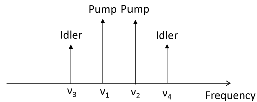
Fig. 1. Schematic spectrum of frequency components generated for partially degenerated FWM.
