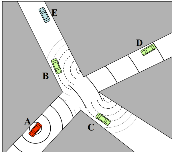
Fig. 10. Vehicles in non-line-of-sight are able to receive the message through reflection and diffraction if they are close enough to a junction.
