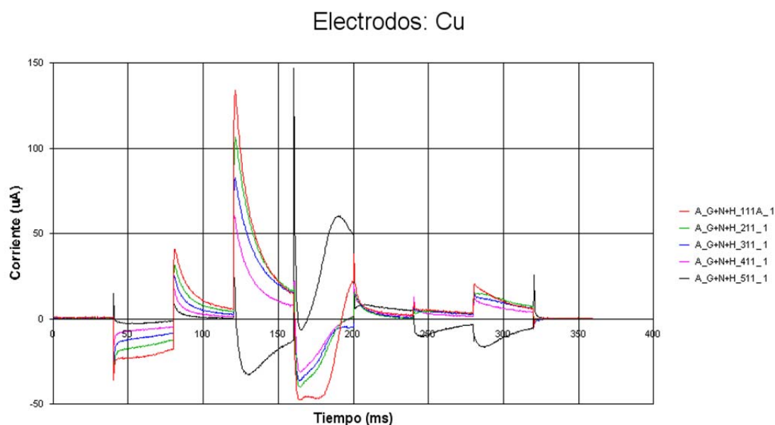
Figure 3.- Electrochemical responses for voltammetric assays to five different Glyphosate concentrations measured with copper electrode.
