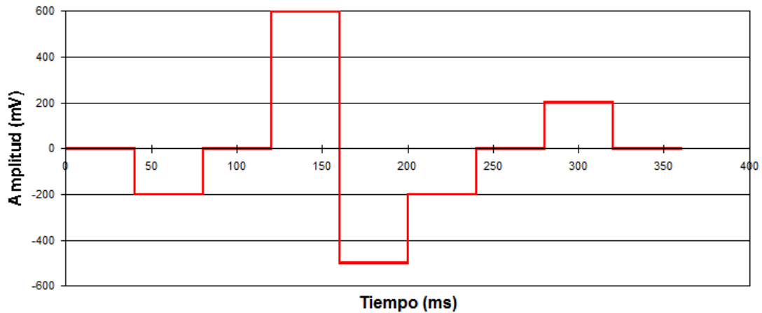
Figure 2.- Pulse train used to carry out the experiences with pulsed voltammetry.
