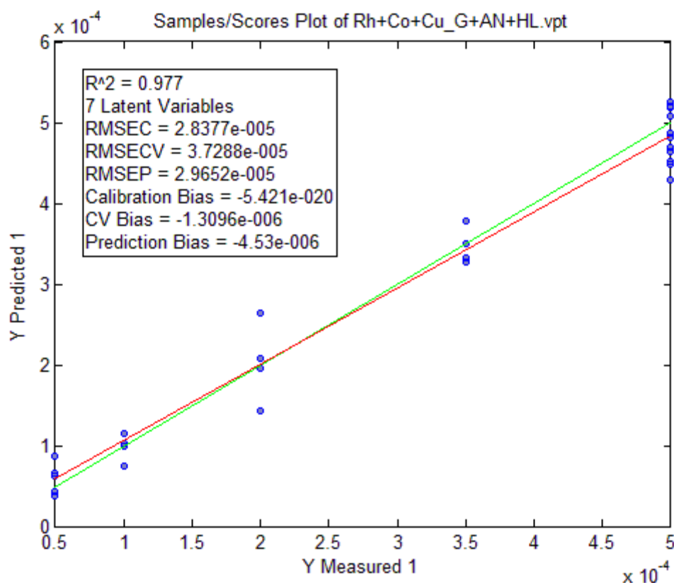
Figure 4.- Measured versus predicted results for Glyphosate concentrations of the model built with Solo © for a combination of the data from rhodium, copper, and cobalt electrodes.
