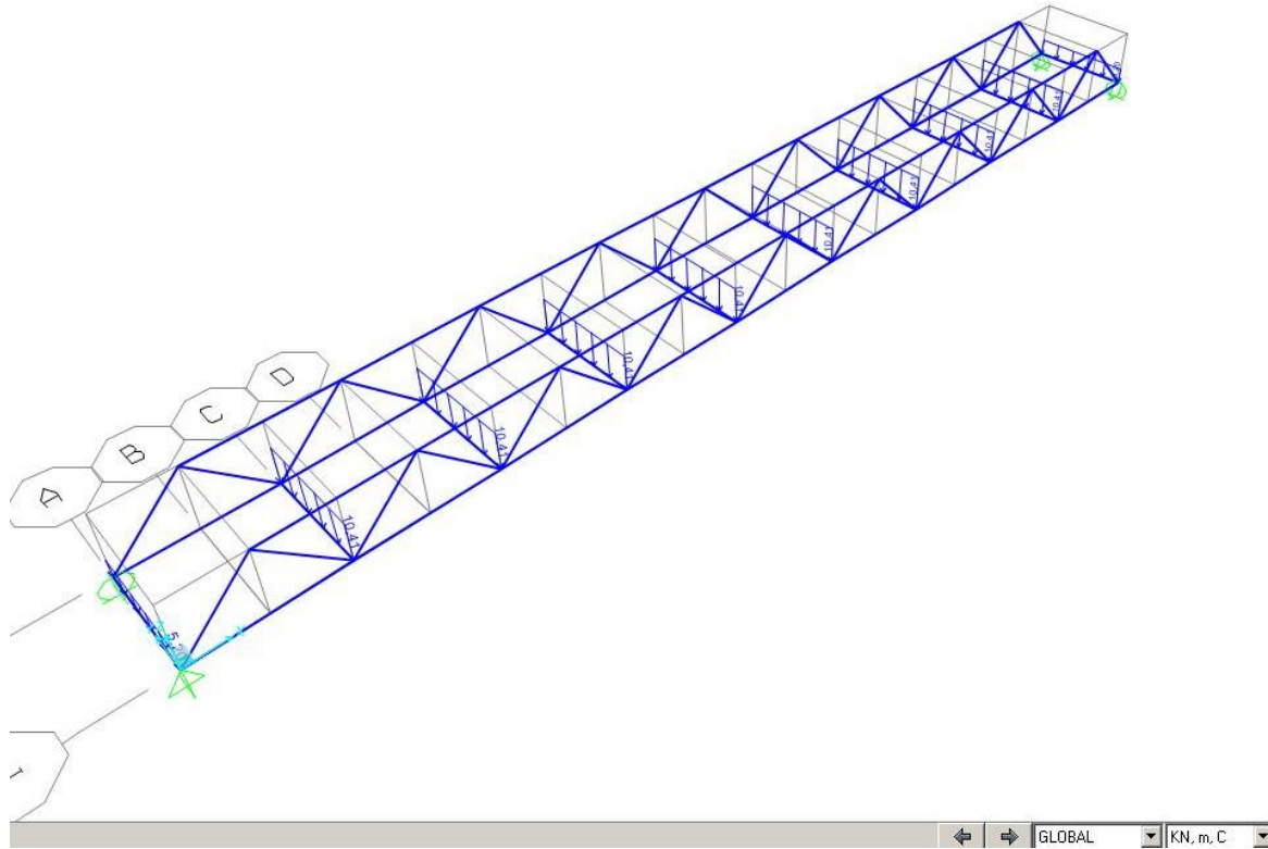
Figura 6: Agua (24,997 kN/m)
