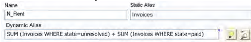
Fig. 4. Example of modelling MoU_SSF2 in the Abstract Interaction Model
