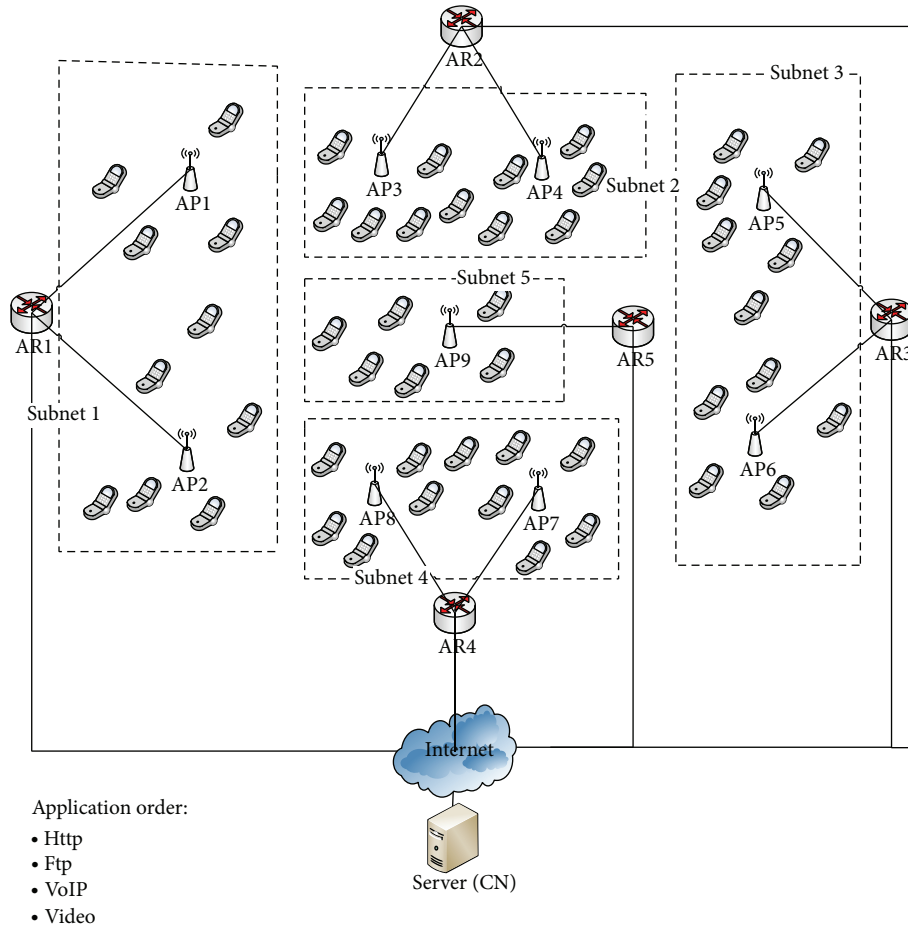
(a) Design of simulation scenario
