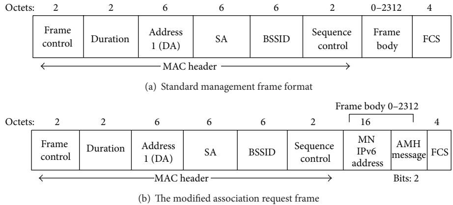
FIGURE 3: The management frame format and modified association request frame.
