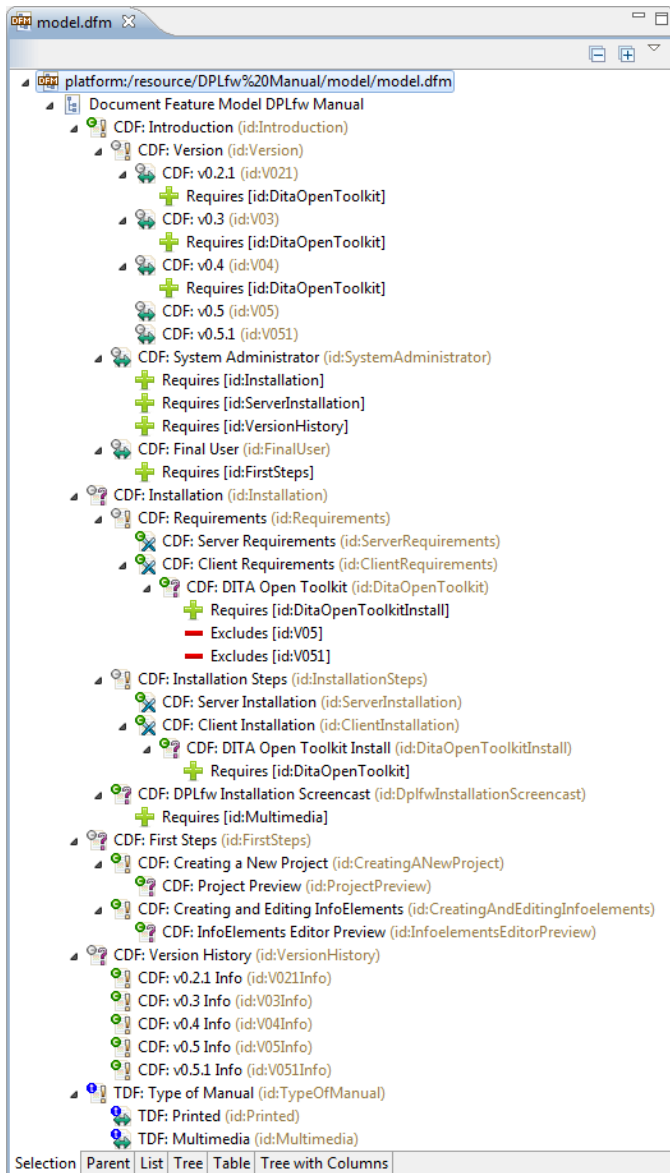
Figure 9: Feature Editor
