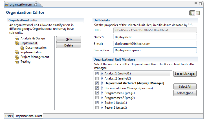
Figure 4: Organization Editor
