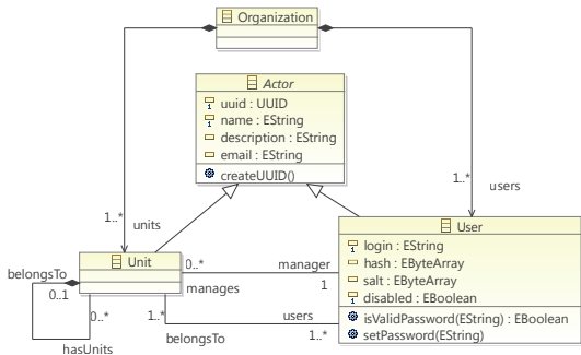
Figure 3: Organizational Model
