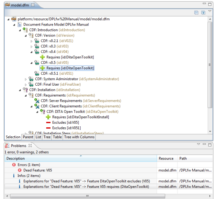
Figure 10: Feature Editor and Problems View
