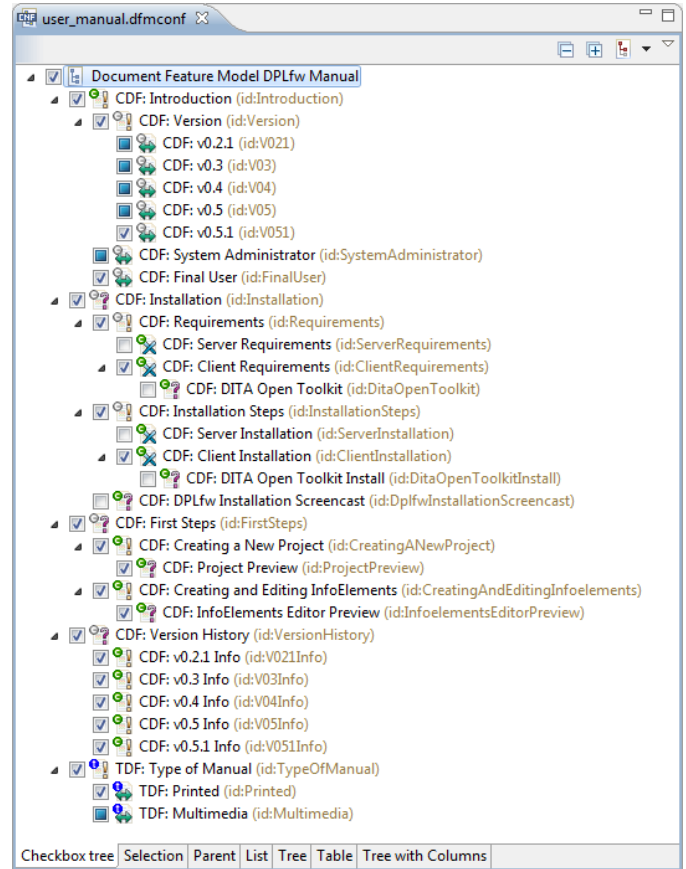
Figure 12: Configuration Editor
