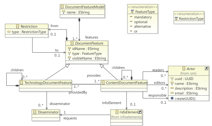
Figure 8: Feature metamodel
