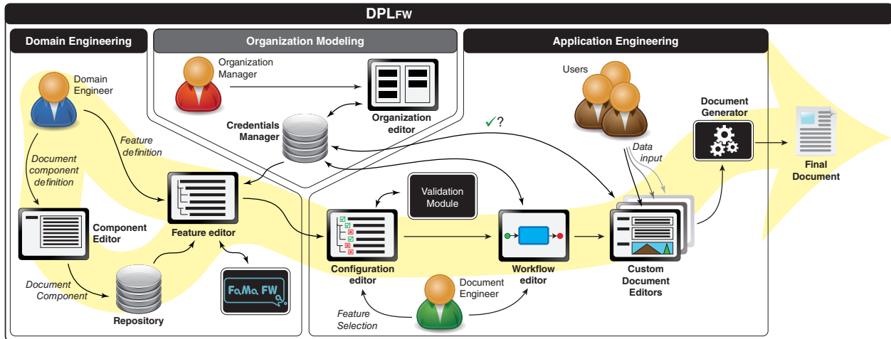
Figure 2: DPLFW overview
