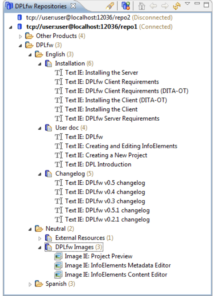
Figure 6: Repository Explorer
