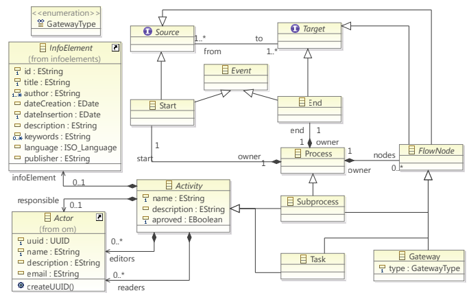
Figure 13: Workflow metamodel
