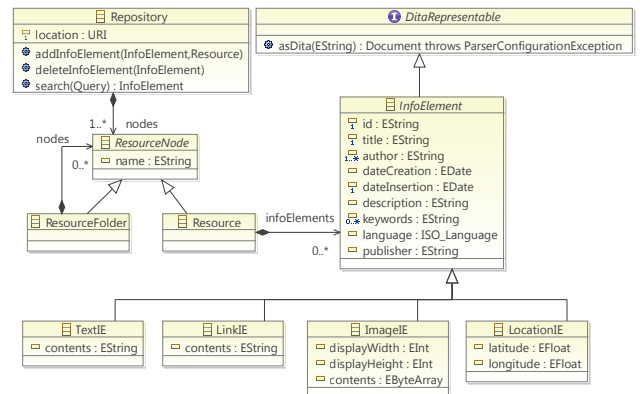
Figure 5: Repository Model
