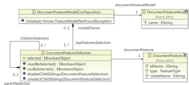
Figure 11: Document Configuration Metamodel
