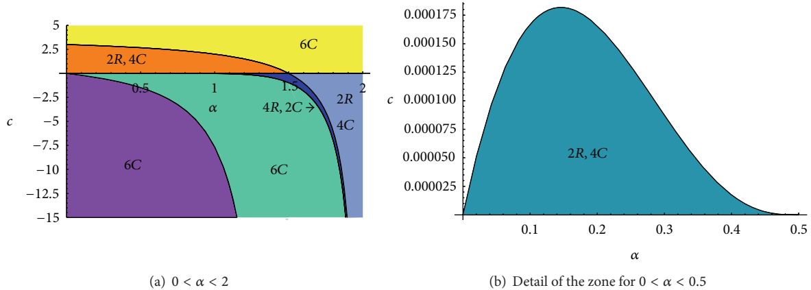
FIGURE 6: Critical points in the (\alpha, c) -plane for 0 < \alpha < 2 .
