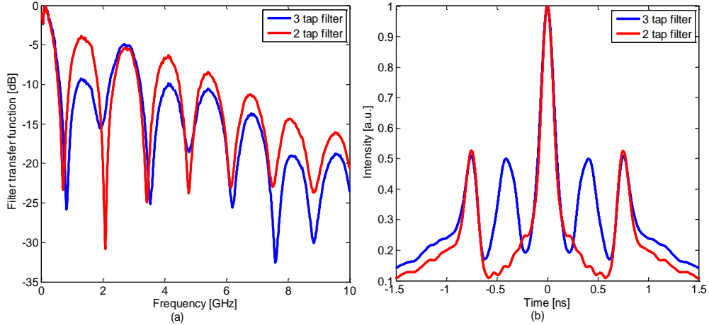
Fig. 4. a) Frequency response of three tap and two tap filters obtained by placing two hot-spots and one hot-spot along the grating, respectively. Fig. 4. b) Inverse Fourier transforms of the amplitude of the MWP filters shown in Fig. 4(a).
