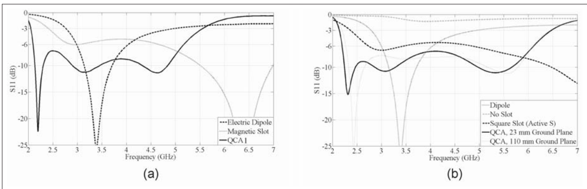
■ Figure 3. Simulated reflection coefficient of the antenna structures presented in Fig. 1: (a) QCA1 and (b) QCA2.
