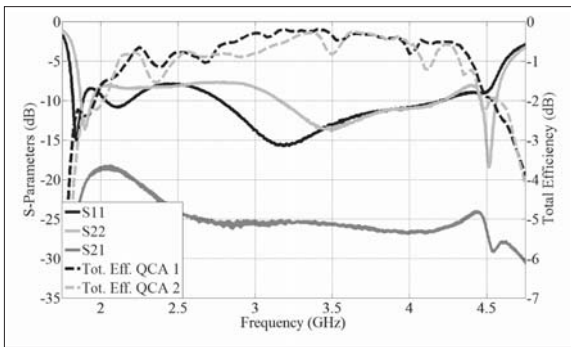
■ Figure 7. Measured S-parameters and total efficiency of QCA 1 and QCA 2 shown in Fig. 5.
