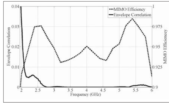
■ Figure 17. Measured envelope correlation and MIMO multiplexing efficiency of the antenna shown in Fig. 14.
