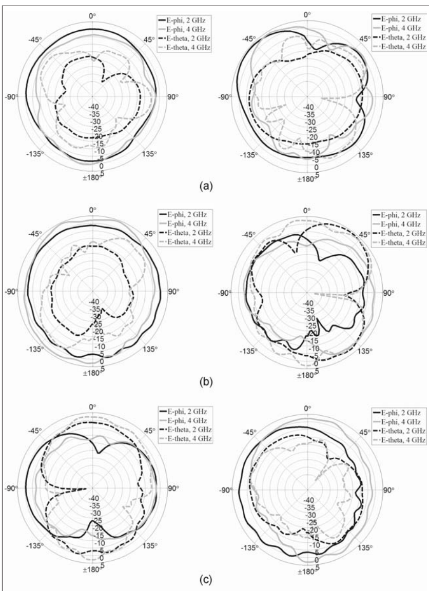
■ Figure 8. Radiation patterns (in dB) for Phi and Theta components at 2 GHz and 4 GHz in (a) XY-cut, (b) XZ-cut, and (c) YZ-cut. The legend of the lines is as follows: (—) E-phi at 2 GHz, (---) E-phi at 4 GHz, (- - -) E-theta at 2 GHz, and (- - -) E-theta at 4 GHz.
