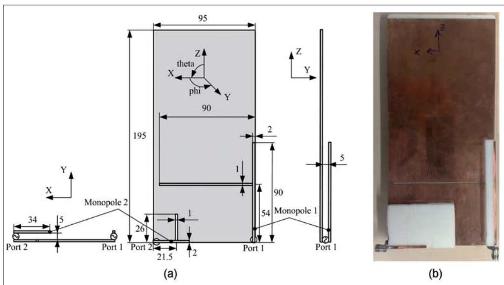
■ Figure 10. (a) Planar radiating ground plane with monopoles of two different lengths as coupling elements. The gray color is metal, whereas the white color is air. Dimensions are in mm. (b) Prototype of the antenna.
