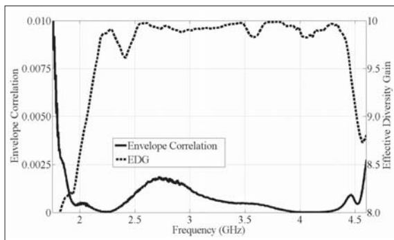
■ Figure 9. Measured envelope correlation and effective diversity gain.
