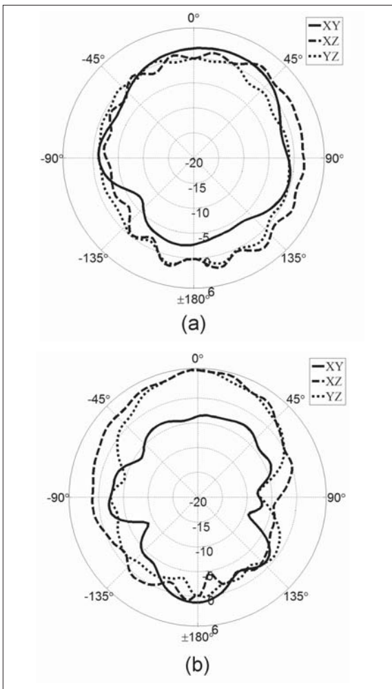
■ Figure 16. Measured radiation patterns of QCA 2 at (a) 2 GHz and (b) 5 GHz in terms of total gain (dBi). GHz and 5 GHz, respectively.
