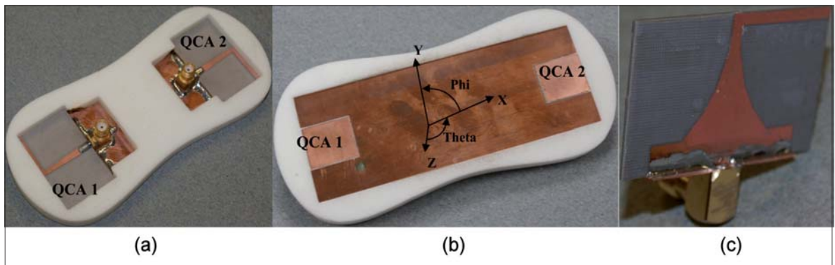
■ Figure 14. Picture of the MIMO antenna prototype: (a) Upper view; (b) Bottom view. The ground plane of the tapered microstrip line balun is presented in (c).
