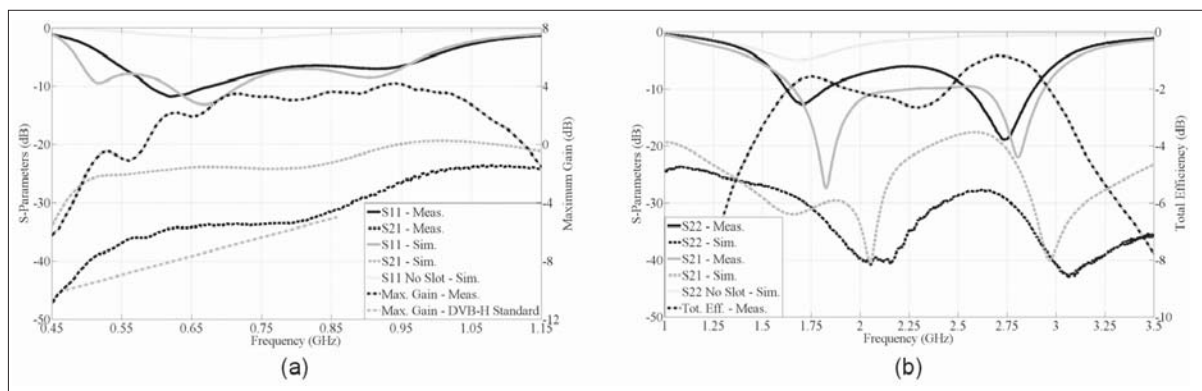
■ Figure 11. Measured and simulated S-parameters (a) for Monopole 1, with measured maximum gain and (b) for Monopole 2, with measured total efficiency. Simulated S-parameters are compared with the case without slot.
