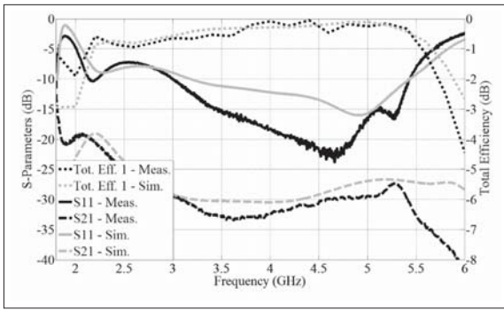
■ Figure 15. Simulated and measured S-parameters (dB), and measured total efficiency (dB).
