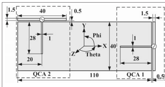
■ Figure 5. Polarization diversity antenna with two orthogonal quasi-complementary antennas. Dimension are in mm.
