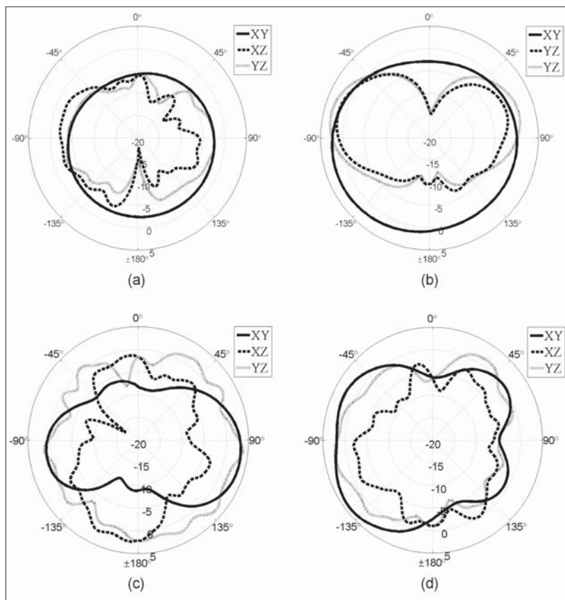
■ Figure 12. Measured radiation patterns in total gain at (a) 500 MHz, (b) 900 MHz, (c) 1.70 GHz, and (d) 2.75 GHz.
