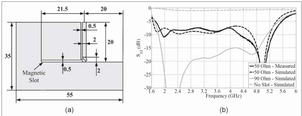
■ Figure 4. (a) Novel basic antenna combining an electric monopole and a magnetic notch. Dimensions in mm. (b) Measured and simulated reflection coefficient and comparison to the cases with 90 \Omega reference input impedance and without magnetic slot.
