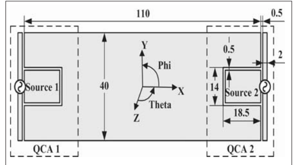
■ Figure 13. MIMO prototype antenna with two QCA basic structures at both end of the ground plane. Dimensions are in mm.
