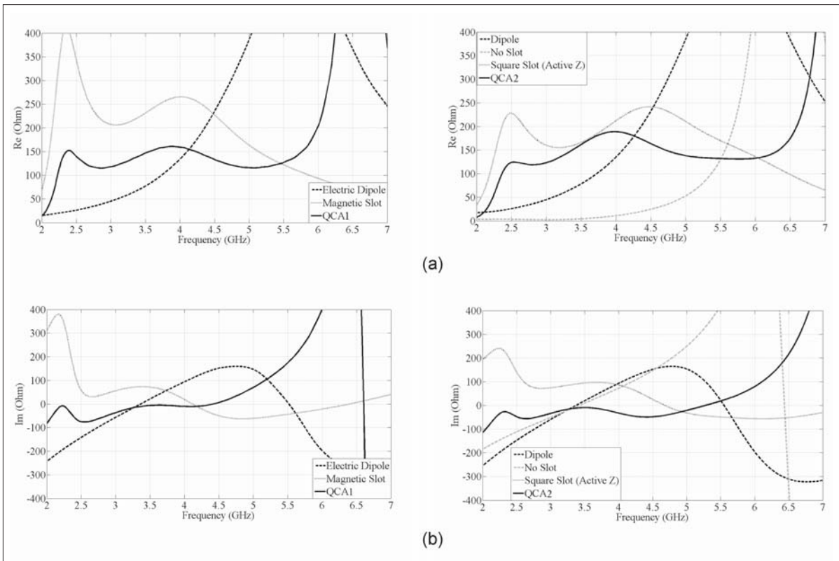
■ Figure 2. Simulated (a) real part and (b) imaginary part of the input impedance of the antenna structures presented in Fig. 1 (a) (left) and Fig. 1(b) (right).
