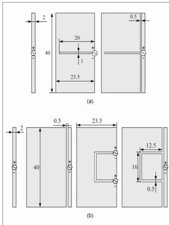
■ Figure 1. Basic wideband radiating structures with (a) a notch (QCA1) and (b) a square-shaped slot (QCA2). Antenna structures to be compared with the basic structures are presented in the same figure.
