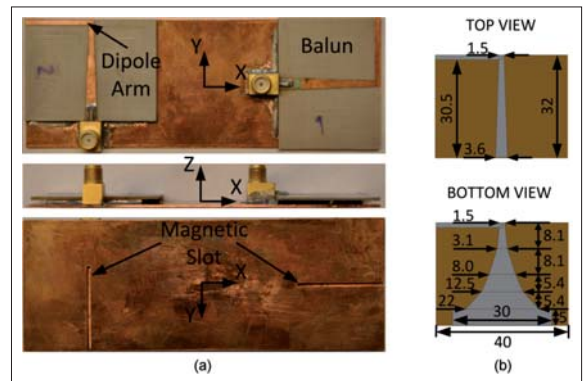
■ Figure 6. (a) Polarization diversity antenna prototype (top view, side view and bottom view); (b) Balun topology.
